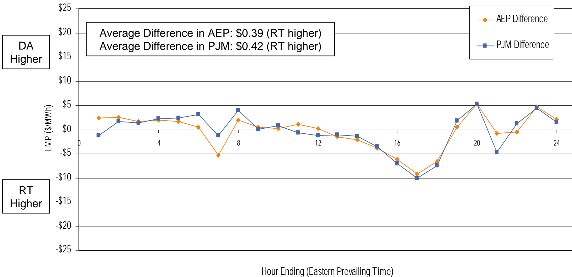
Average hourly difference of day-ahead and real-time LMPs April 2006
