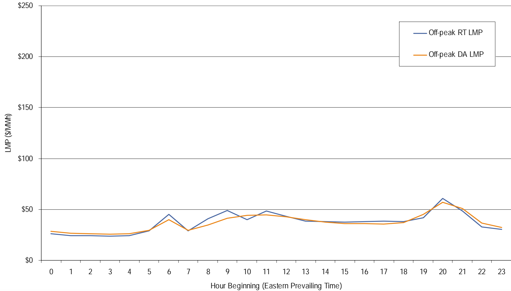
AEP real-time and day-ahead hourly average off-peak LMP April 2006
