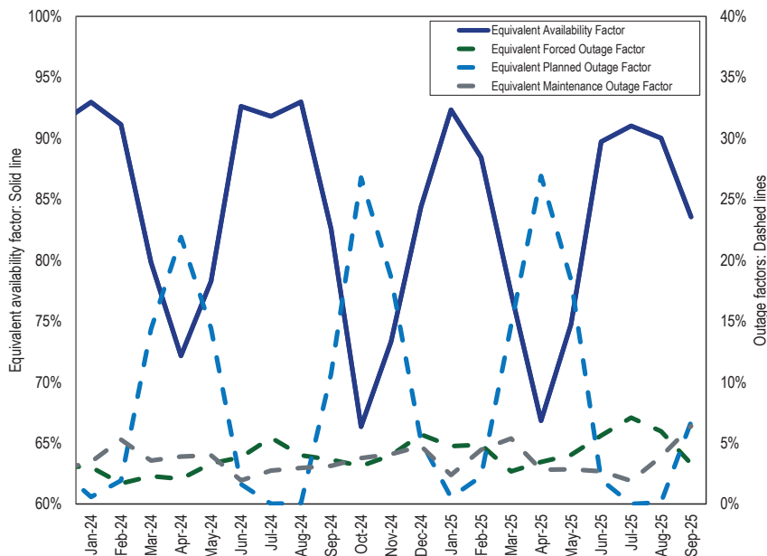
Figure 5-13 Monthly generator performance factors: January through September, 2024 through 2025
