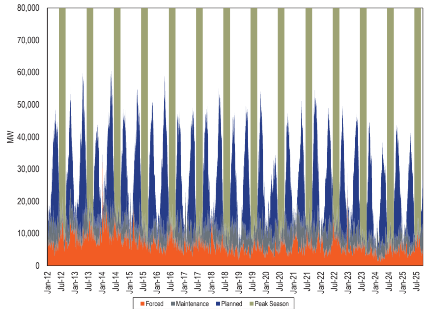
Figure 5-10 Outages (MW): 2012 through September 2025
