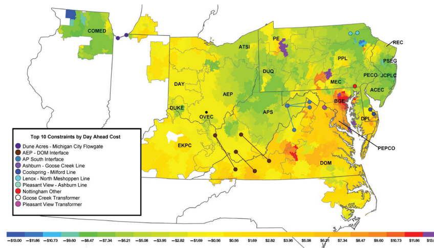
Figure 11-9 Location of top 10 constraints by day-ahead congestion costs: January through September, 2025
