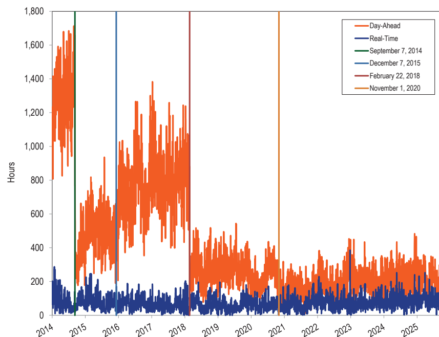
Figure 11-10 Daily congestion event hours: January 2014 through September 2025
