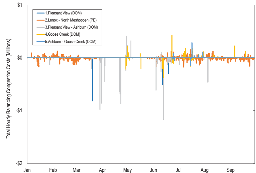
Figure 11-5 Top five constraints affecting balancing congestion costs: January through September, 2025
