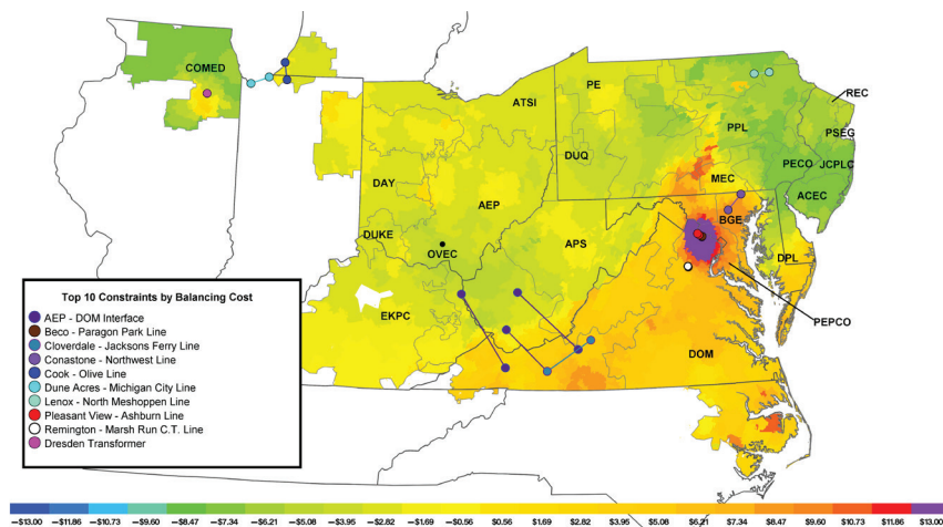
Figure 11-8 Location of top 10 constraints by balancing congestion costs: January through September, 2025
