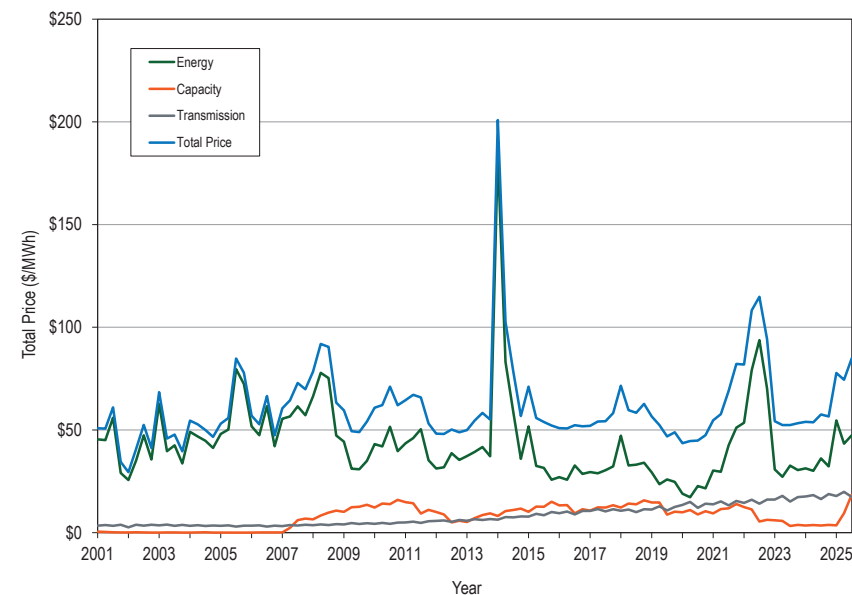
Figure 1-4 Top three components of quarterly total cost ($/MWh): January 2001 through September 2025 62
