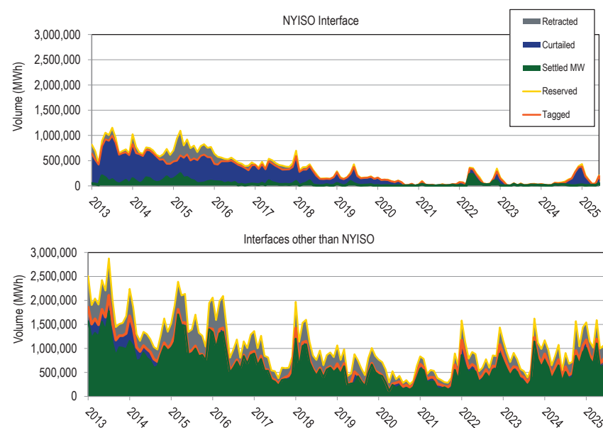
Figure 9–13 Spot import service use: January 2013 through June 2025
