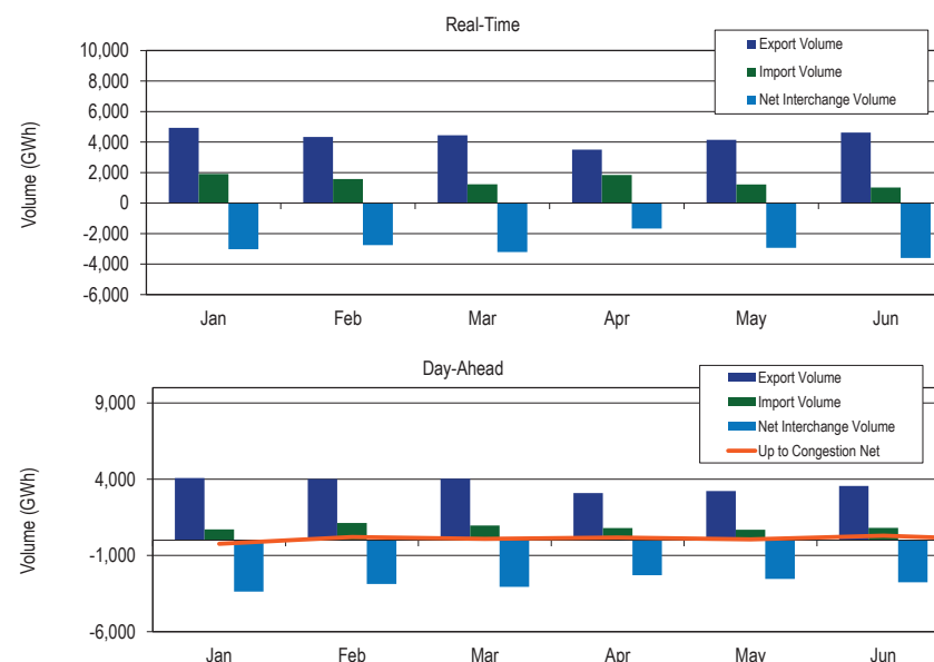
Figure 9-1 Scheduled imports and exports: January through June, 2025
