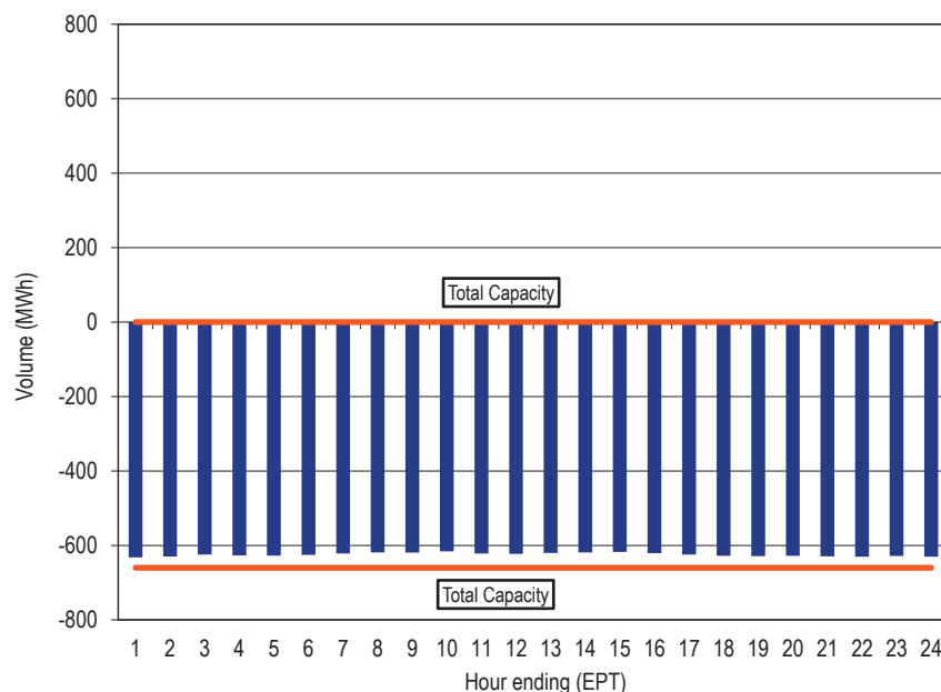
Figure 9-7 Neptune hourly average flow: January through June, 2025
