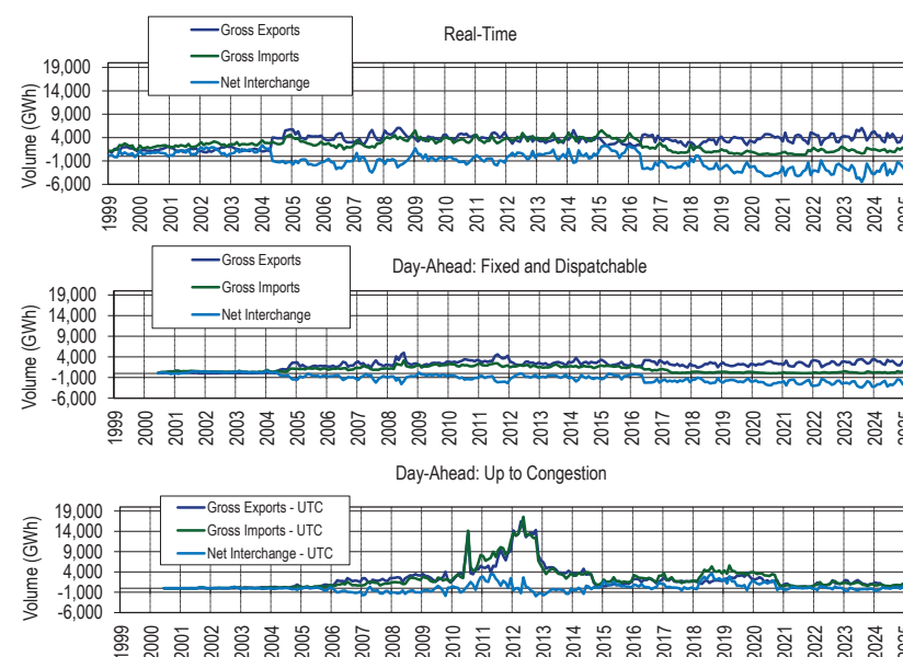
Figure 9-2 Scheduled import and export transaction volume history: January 1, 1999 through June 30, 2025
