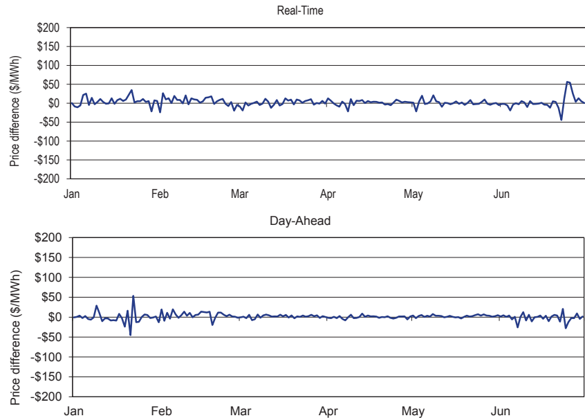
Figure 9-6 Price differences (NY/PJM proxy – PJM/NYIS Interface): January through June, 2025
