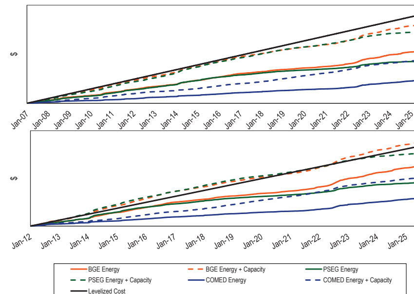
Figure 7-5 Historical new entrant CC revenue adequacy: 2007 through June 2025 and 2012 through June 2025 26
