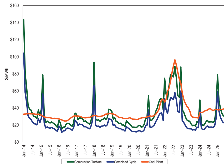
Figure 7-4 Average short run marginal costs: 2014 through June 2025
