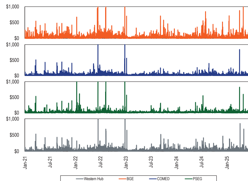
Figure 7-2 Hourly spark spread (gas) for peak hours ($/MWh): 2021 through June 2025 2
