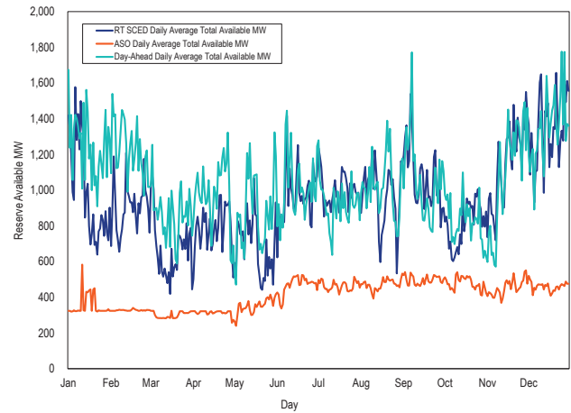
Figure 10-25 Daily average total available MW in the day-ahead, ASO, and RT SCED solutions: 2024
