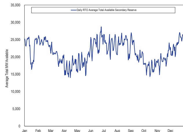
Figure 10-29 Daily Average Available Secondary Reserve: 2024
