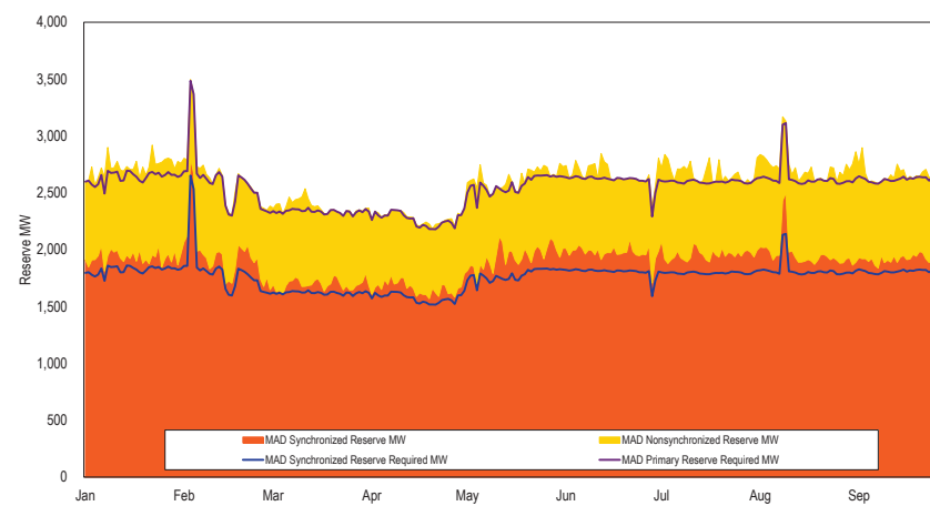
Figure 10-7 Daily average real-time MAD reserve products and daily average real-time MAD reserve service requirements: January through September, 2023
