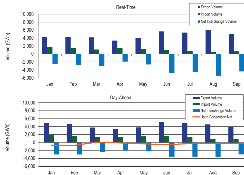
Figure 9-1 Scheduled imports and exports: January through September, 2023
