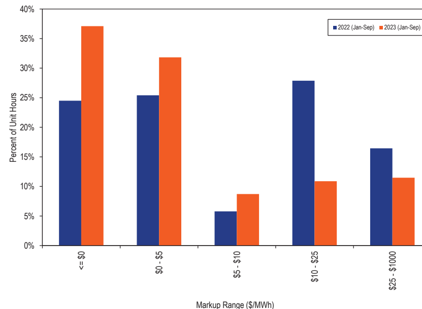
Figure 3-64 Frequency distribution of highest markup of coal units offered using unadjusted cost offers: January through September, 2022 and 2023
