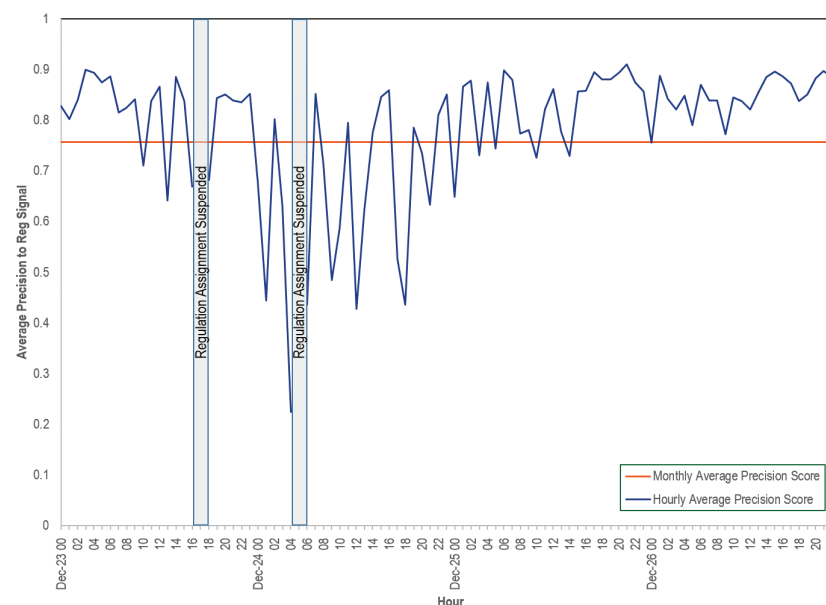
Figure 10-36 Average hourly and rest of month RegD precision score of battery units
