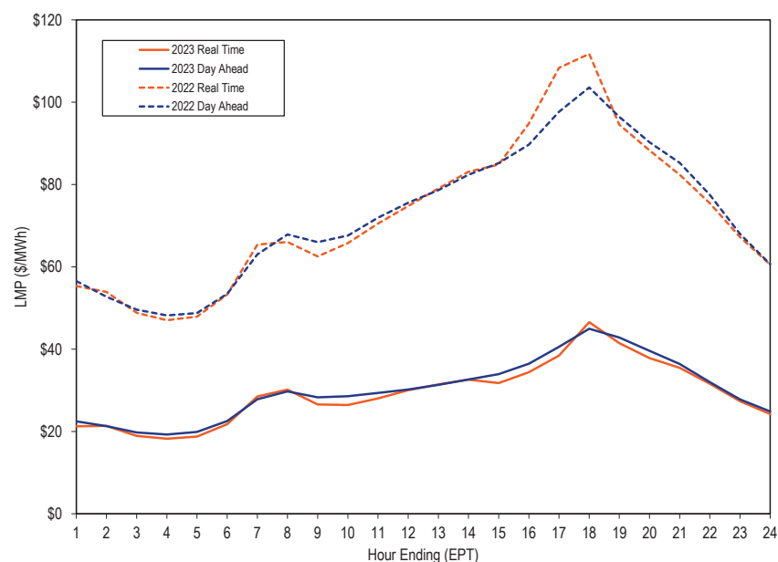
Figure 3-43 System hourly average LMP: January through September, 2022 and 2023
