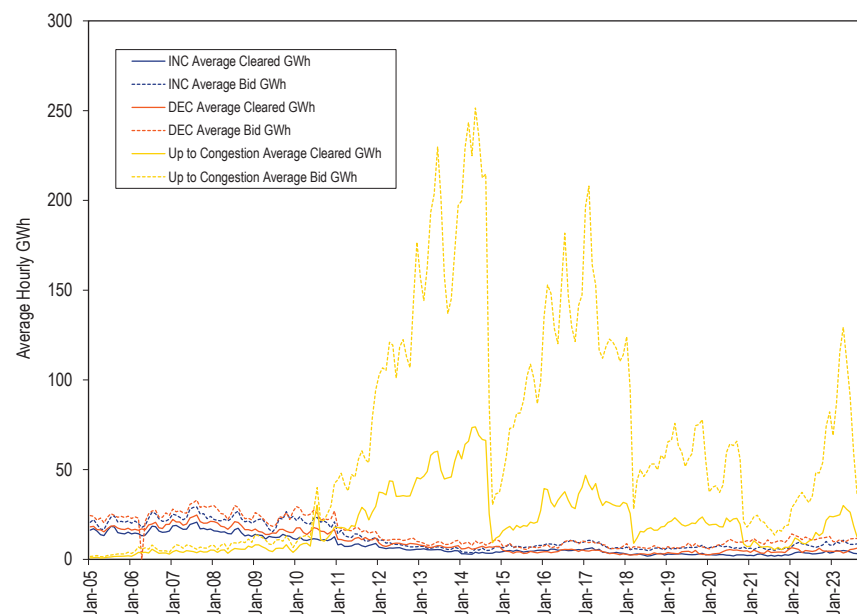
Figure 3-20 Monthly bid and cleared INCs, DEC and UTCs (GWh): January 2005 through September 2023
