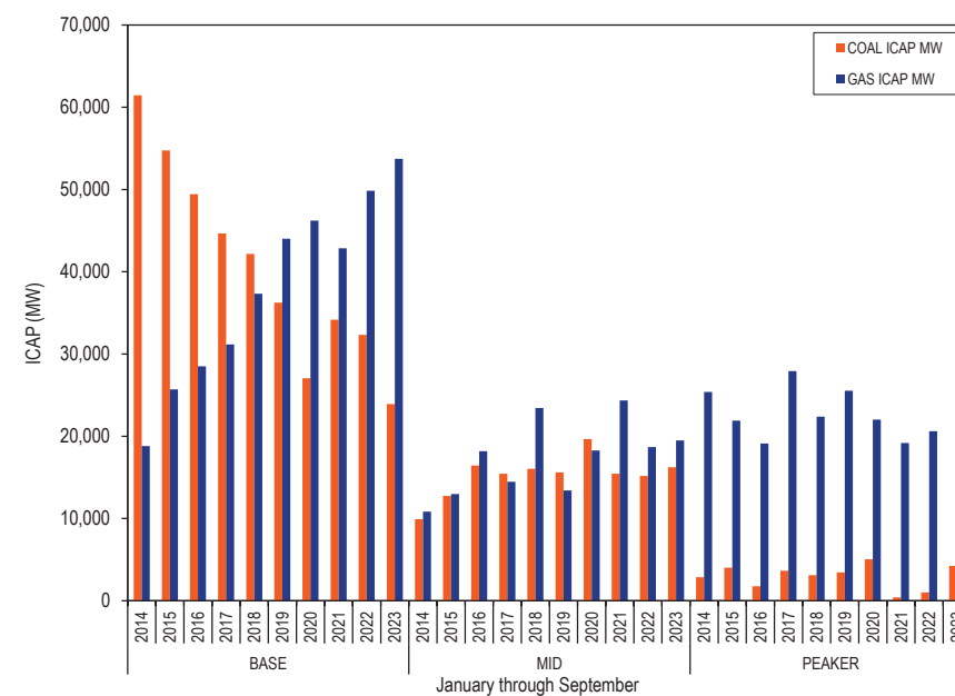
Figure 3-56 Real-time annual gas and coal unit segment classification: January through September, 2014 through 2023
