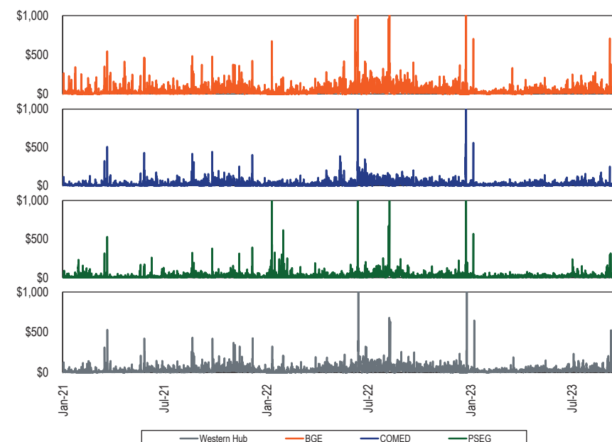
Figure 7-2 Hourly spark spread (gas) for peak hours ($/MWh): 2021 through September 2023 2
