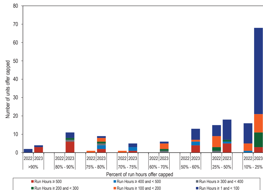
Figure 3-62 Real-time offer capped unit statistics: January through September, 2022 and 2023
