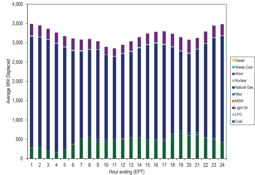
Figure 8-17 Marginal fuel at time of wind generation: January through September, 2023
