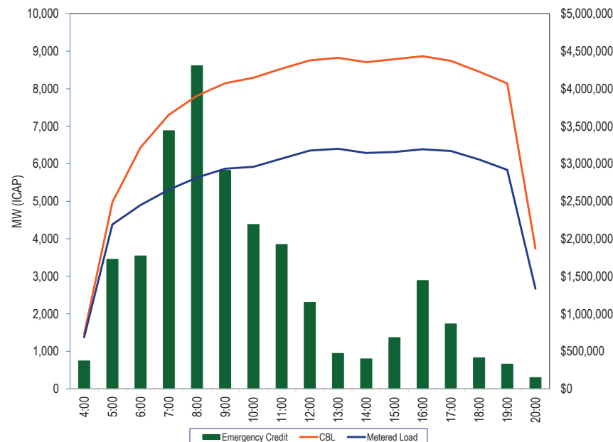
Figure 6-10 Emergency energy credits, CBL and metered load: December 24, 2022
