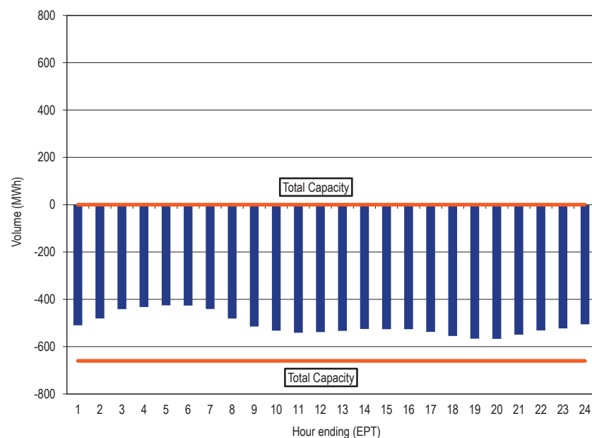
Figure 9-6 Neptune hourly average flow: January 1 through June 30, 2017
