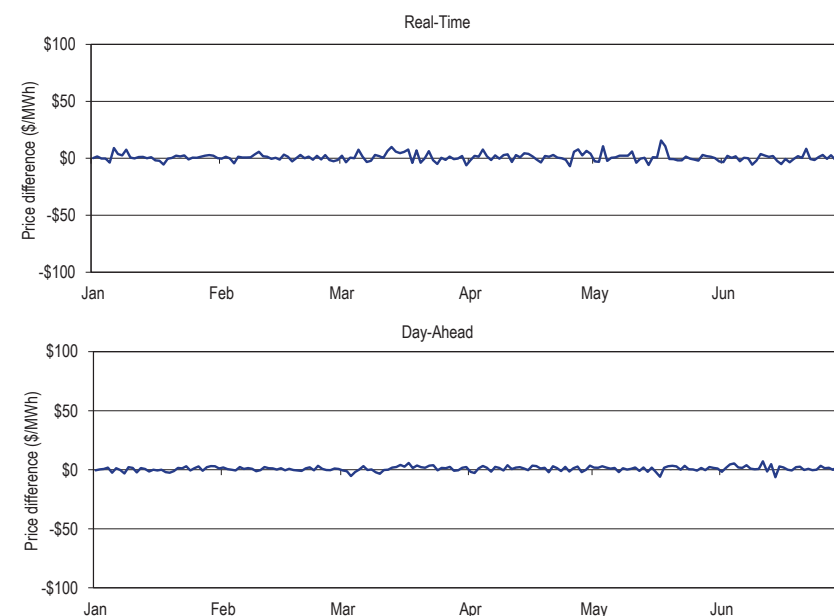
Figure 9-4 Real-time and day-ahead daily hourly average price difference (MISO/PJM Interface minus PJM/MISO Interface): January 1 through June 30, 2017
