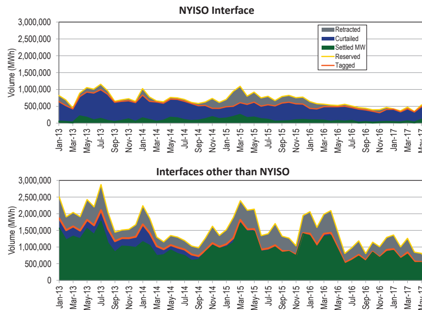
Figure 9-15 Spot import service use: January 1, 2013 through June 30, 2017
