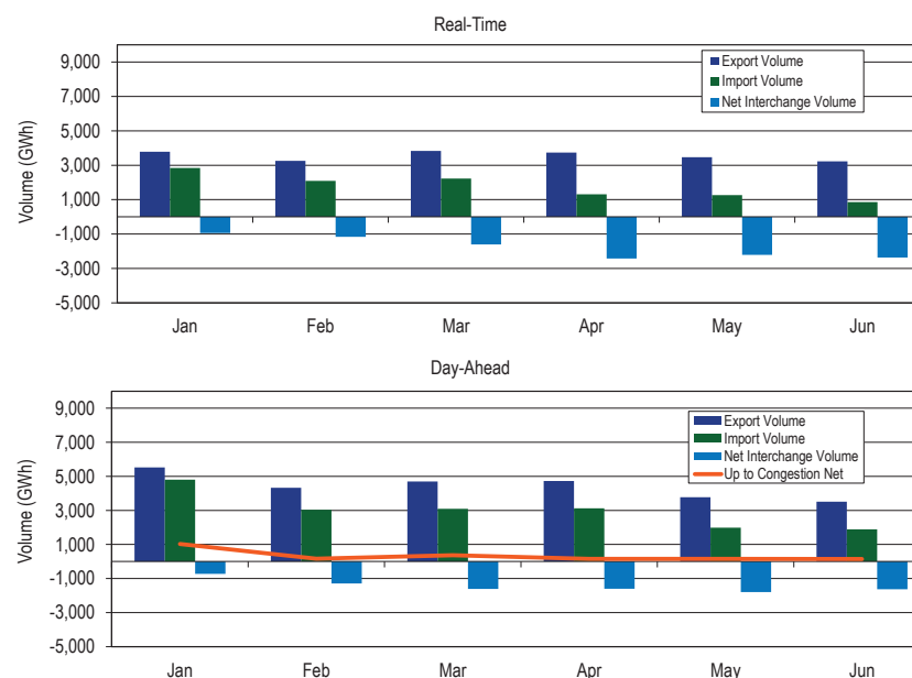
Figure 9-1 PJM real-time and day-ahead scheduled imports and exports: January 1 through June 30, 2017
