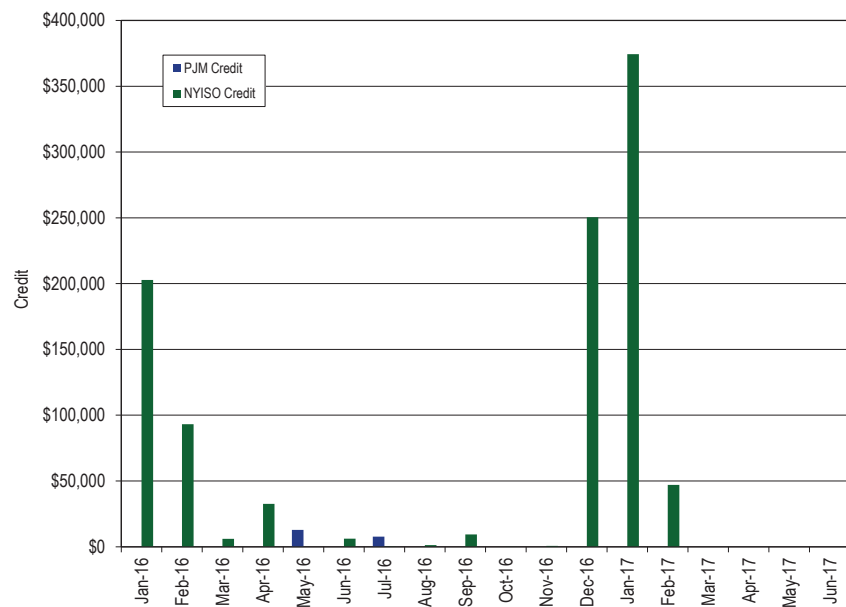
Figure 9-10 Credits for coordinated congestion management (flowgates): January 1, 2016 through June 30, 2017 49
