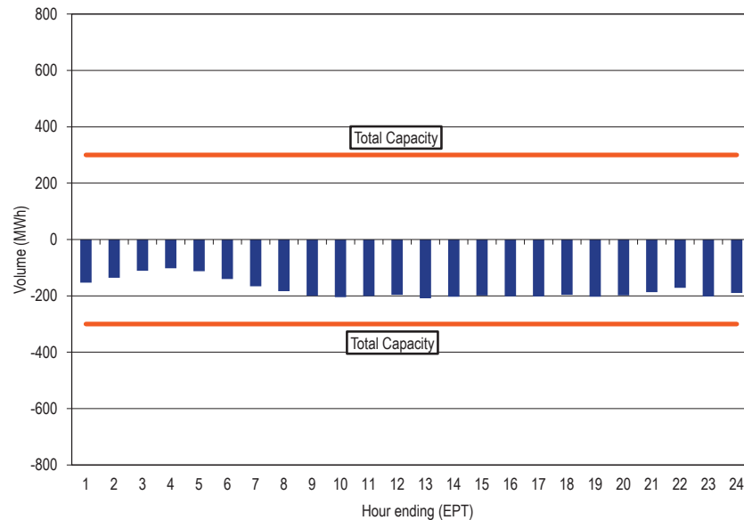
Figure 9-7 Linden hourly average flow: January 1 through June 30, 2017 39
