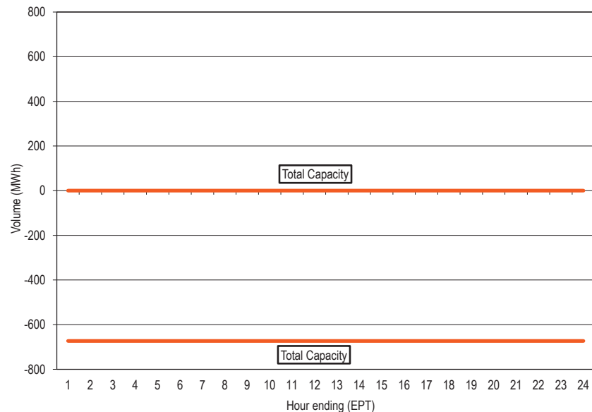
Figure 9-8 Hudson hourly average flow: January 1 through June 30, 2017
