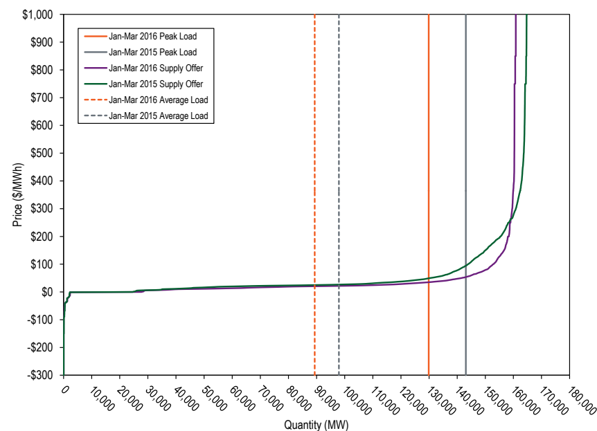
Figure 3-4 Average PJM aggregate real-time generation supply curves by offer price: January through March, 2015 and 2016
