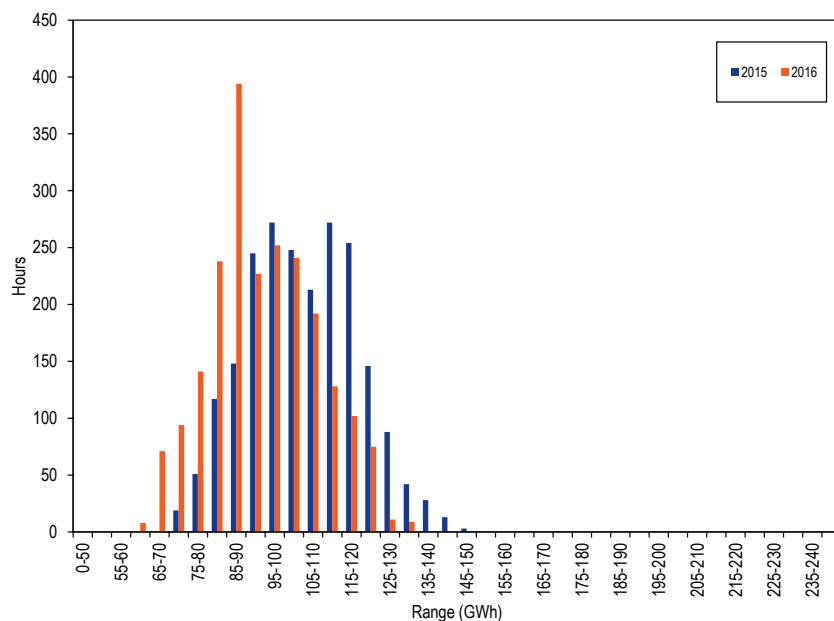
Figure 3-5 Distribution of PJM real-time generation plus imports: January through March, 2015 and 2016 21
