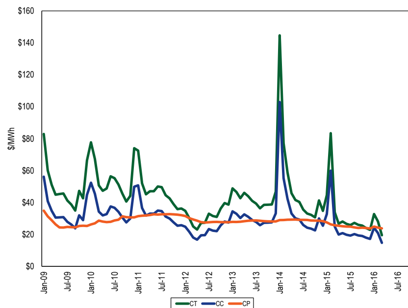
Figure 7-5 Average short run marginal costs: 2009 through March 2016
