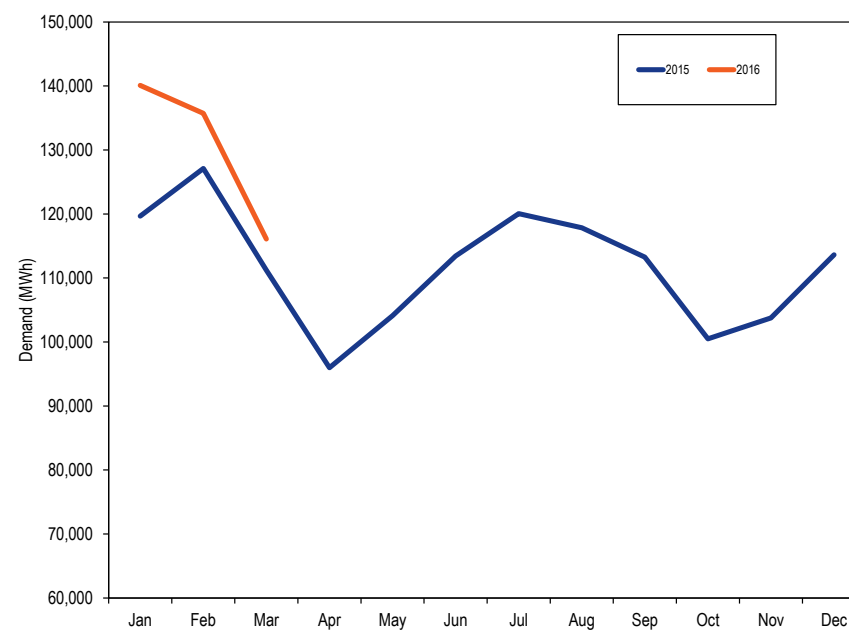
Figure 3-18 PJM day-ahead monthly average hourly demand: January 2015 through March 2016
