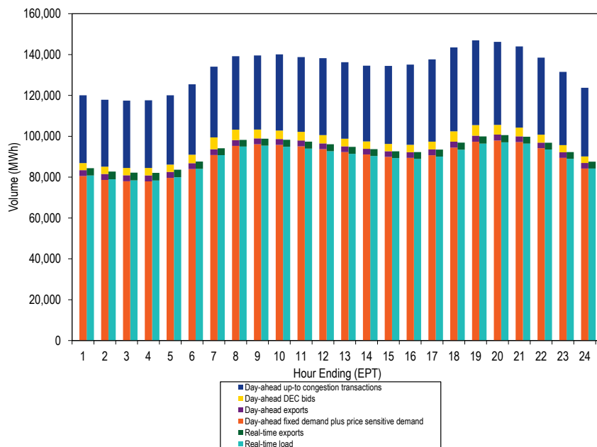
Figure 3-19 Day-ahead and real-time demand (Average hourly volumes): January through March, 2016
