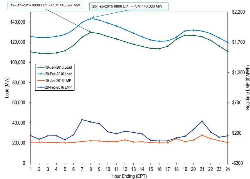
Figure 3-13 PJM peak-load comparison: Tuesday, January 19, 2016 and Friday, February 20, 2015
