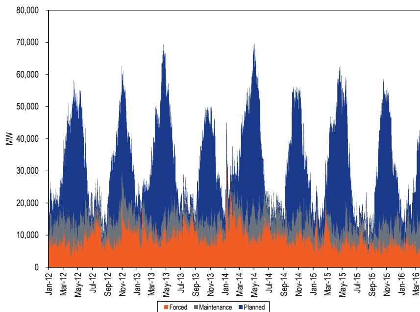
Figure 5-8 PJM outages (MW): 2012 through March 2016
