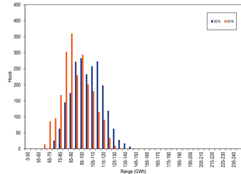
Figure 3-14 Distribution of PJM real-time accounting load plus exports: January through March, 2015 and 2016 30
