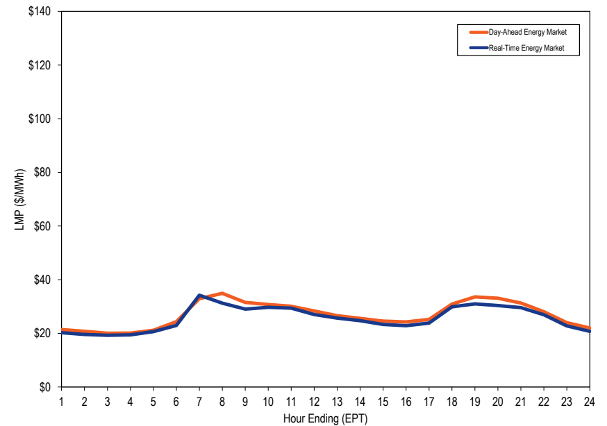
Figure 3-41 PJM system hourly average LMP: January through March, 2016
