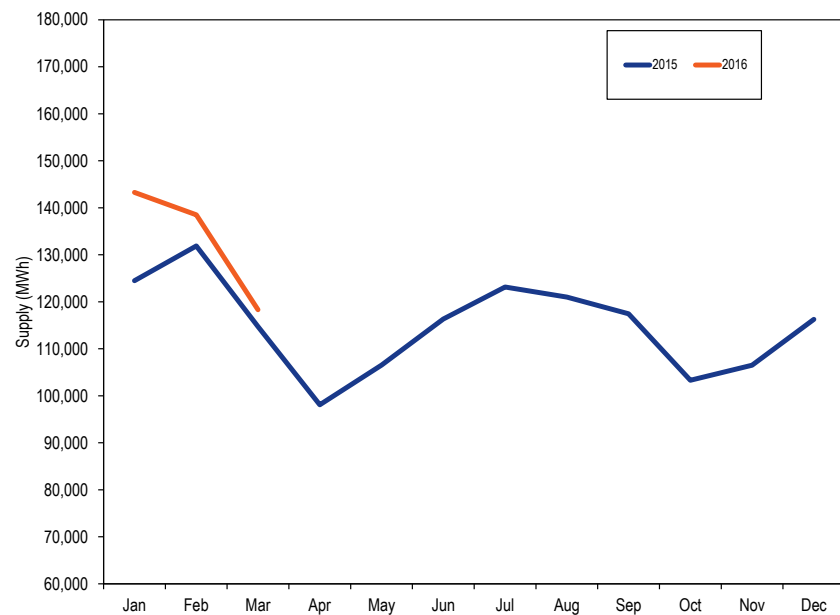
Figure 3-8 PJM day-ahead monthly average hourly supply: January 2015 through March 2016
