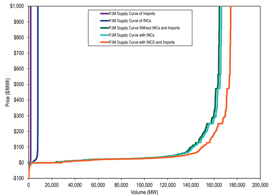
Figure 3-26 PJM day-ahead aggregate supply curves: 2016 example day
