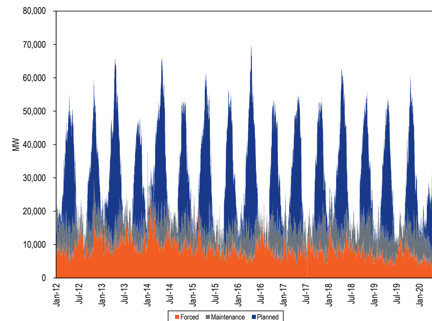
Figure 5-9 Outages (MW): 2012 through June 2020
