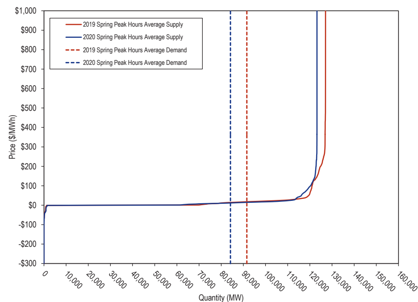
Figure 3-1 Average hourly real-time supply curve comparison: 2019 spring and 2020 spring
