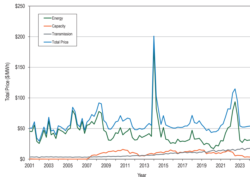
Figure 1-4 Top three components of quarterly total cost ($/MWh): January 2001 through September 2024 56
