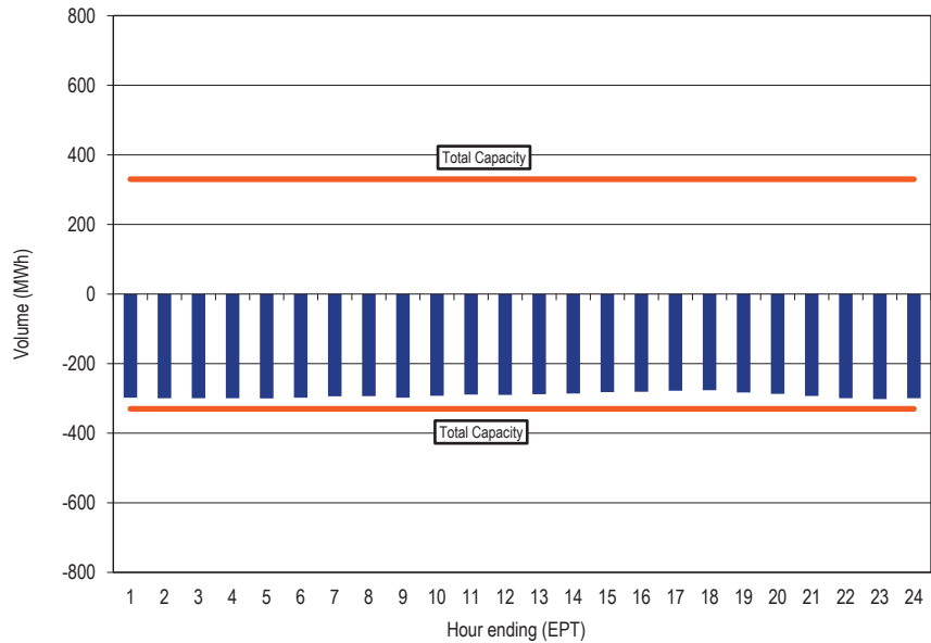
Figure 9-8 Linden hourly average flow: January through September, 2024 31
