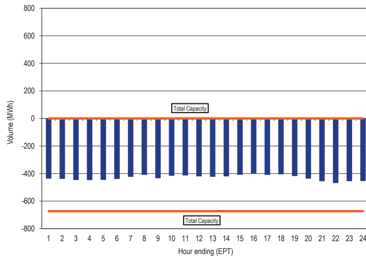
Figure 9-9 Hudson hourly average flow: January through September, 2024
