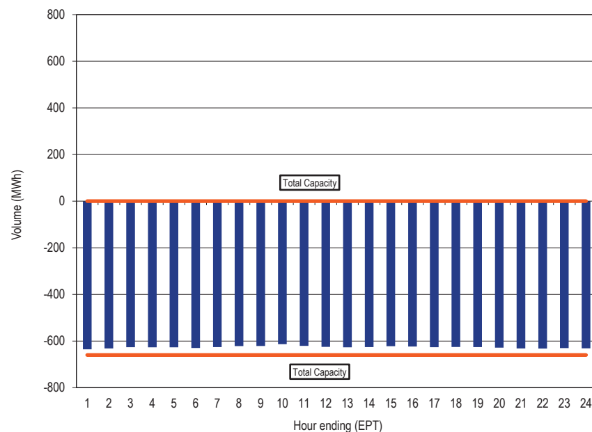
Figure 9-7 Neptune hourly average flow: January through September, 2024
