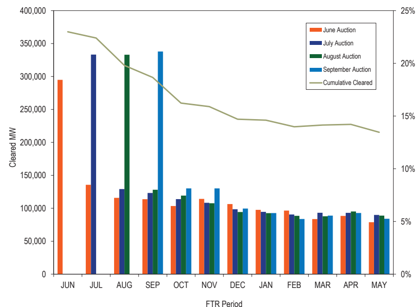
Figure 13-7 Monthly Balance of Planning Period FTR Auction cleared volume (MW per period): June 2024 through September 2024 Auction
