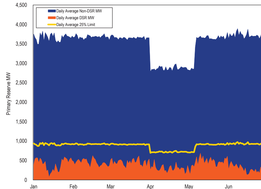
Figure 10-15 Comparison of daily average cleared primary reserve and daily average cleared DSR: January through June, 2024
