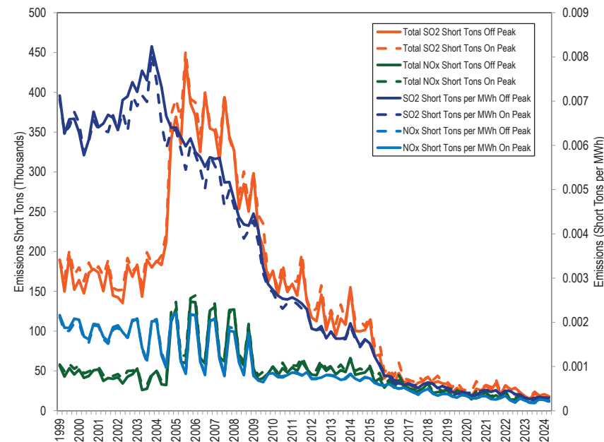
Figure 8-13 SO 2 and NO x emissions during on and off peak hours by quarter (thousands of short tons), by PJM units: January 1999 through June 2024 302
