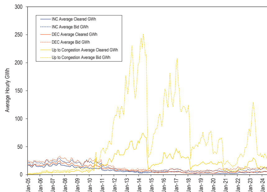
Figure 3-21 Monthly bid and cleared INCs, DEC and UTCs (GWh): January 2005 through June 2024
