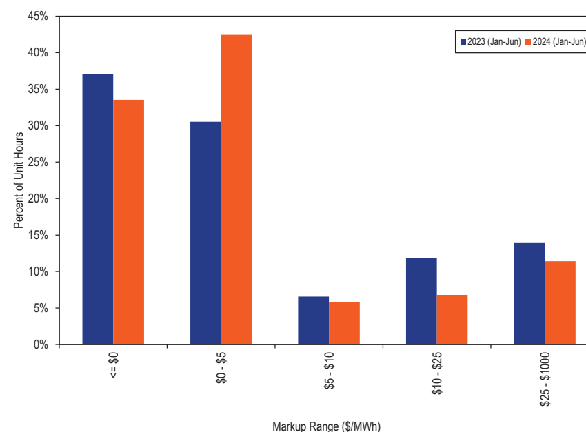
Figure 3-62 Frequency distribution of highest markup of coal units offered using unadjusted cost offers: January through June, 2023 and 2024
