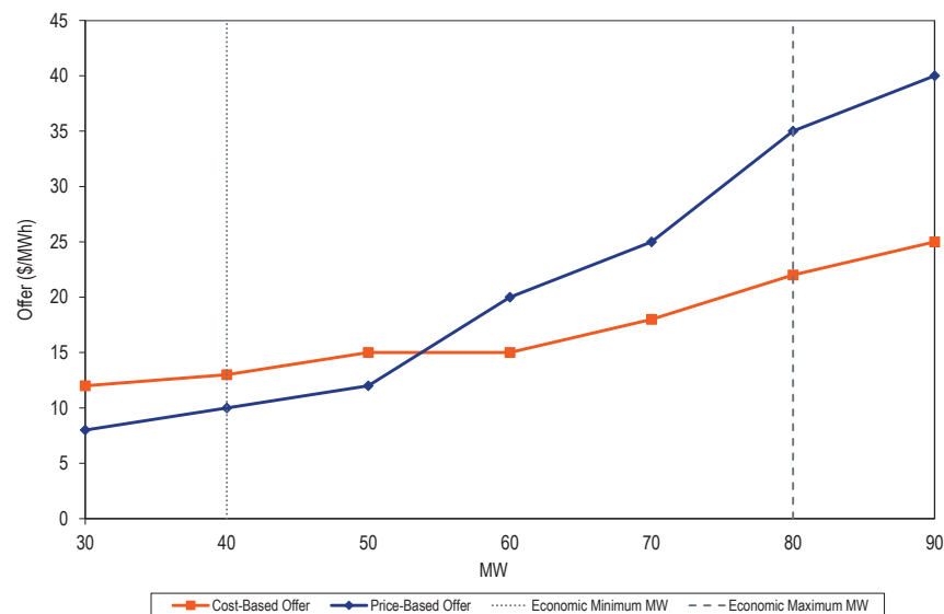
Figure 3-57 Offers with varying markups at different MW output level
