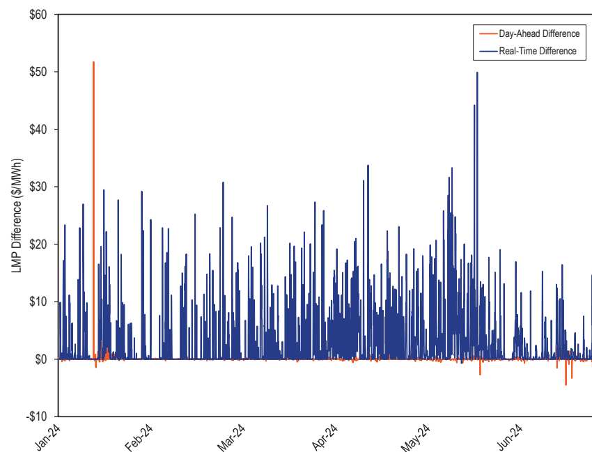
Figure 3-26 Hourly difference between DLMP and PLMP for day-ahead and real-time: January through June, 2024
