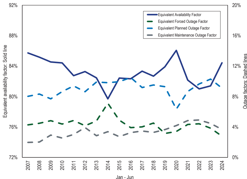
Figure 5-8 Equivalent outage and availability factors: January through June, 2007 to 2024
