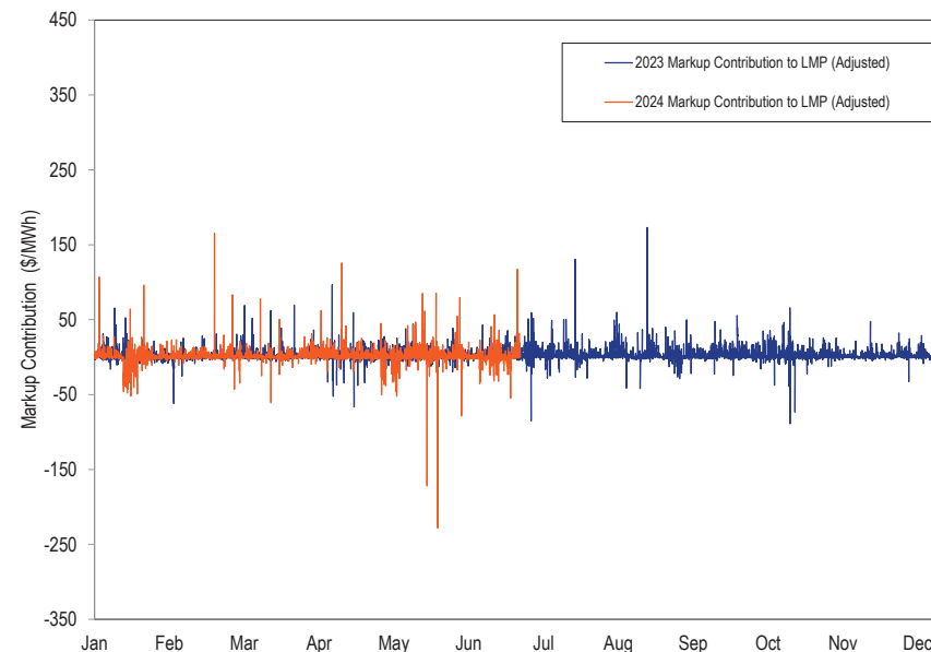
Figure 3-67 Markup contribution to real-time hourly load-weighted LMP (Adjusted): January 2023 through June 2024
