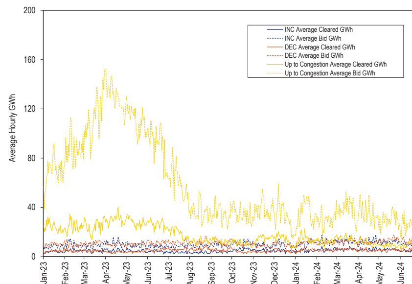
Figure 3-22 Daily bid and cleared INCs, DEC, and UTCs (GWh): January 2023 through June 2024
