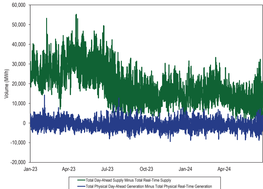
Figure 3-8 Difference between day-ahead and real-time daily average cleared supply: 2023 through June 2024
