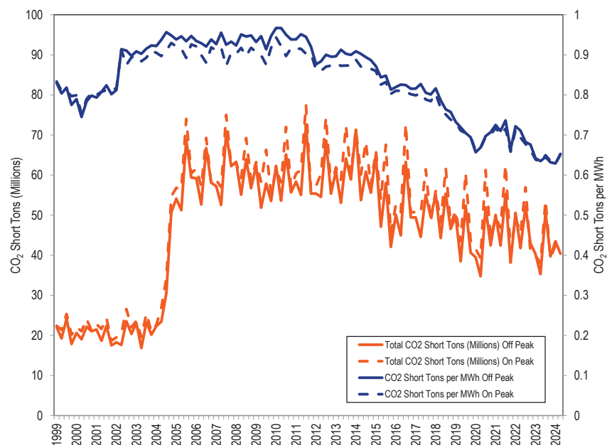
Figure 8-11 Total CO 2 emissions during on and off peak hours by quarter (millions of short tons), by PJM units: January 1999 through June 2024 298
