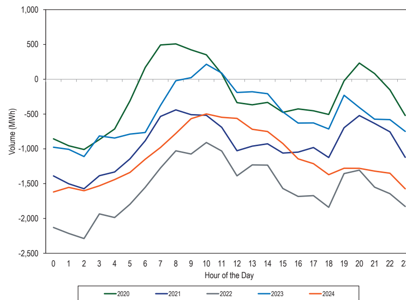
Figure 3-17 Difference between day-ahead and real-time hourly average load by hour of the day (Average hourly volumes): January through June, 2020 through 2024
