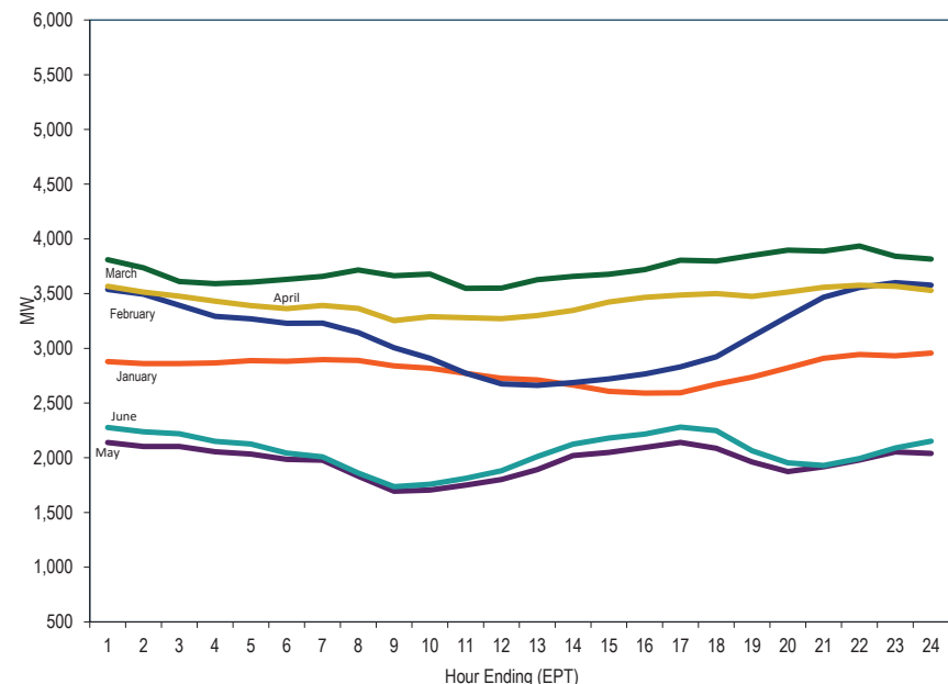
Figure 8-17 Average hourly day-ahead generation of wind units: January through June, 2024
