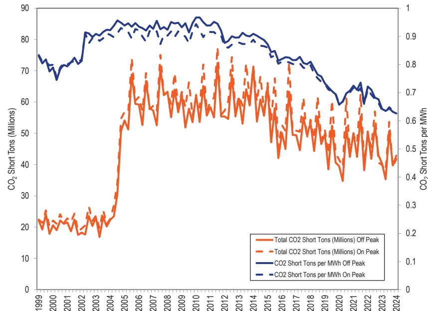
Figure 8-11 Total CO 2 emissions during on and off peak hours by quarter (millions of short tons), by PJM units: January 1999 through March 2024 284
