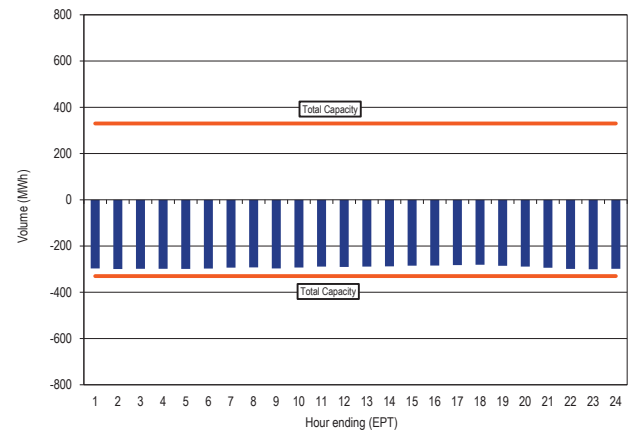
Figure 9-8 Linden hourly average flow: 2024 31
