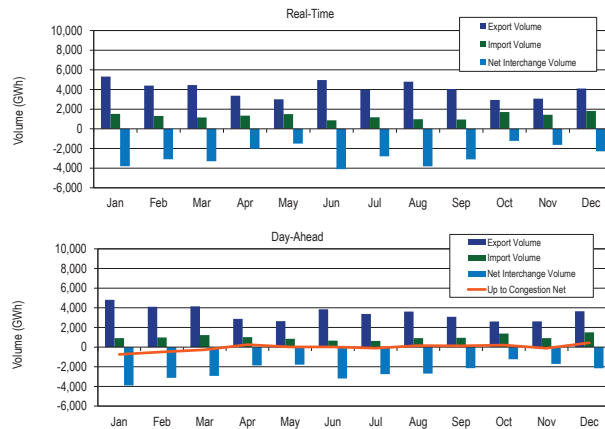
Figure 9-1 Scheduled imports and exports: 2024
