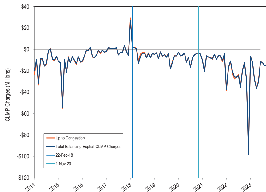
Figure 11-2 Monthly balancing explicit CLMP charges incurred by UTC: January 2014 through September 2023
