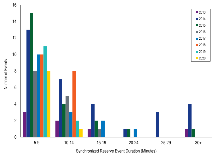
Figure 10-9 Synchronized reserve events duration distribution curve: January 2013 through June 2020
