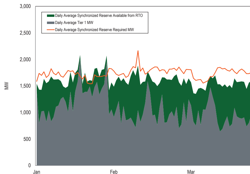
Figure 10-5 Daily average tier 1 synchronized reserve supply (MW) in the MAD Subzone: January through March, 2019
