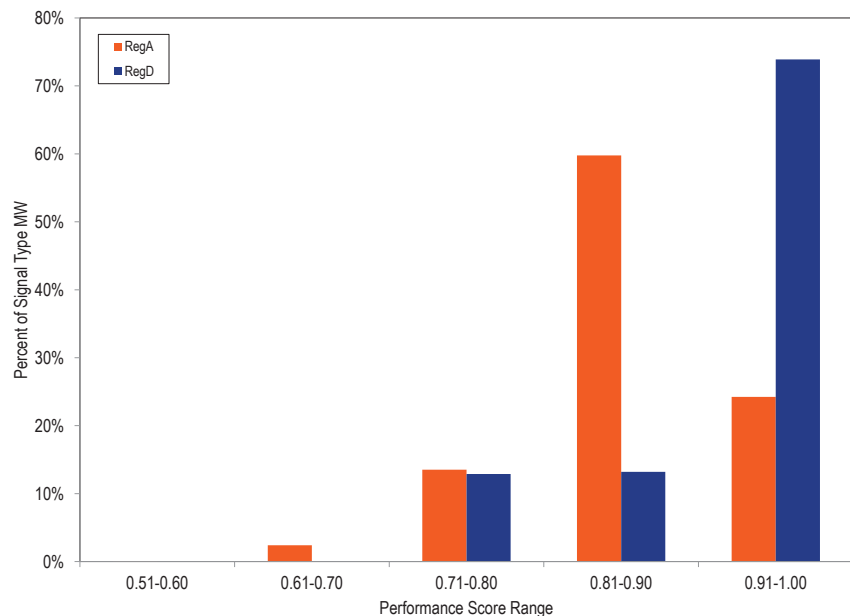
Figure 10-15 Hourly average performance score by regulation signal type: January through March, 2019
