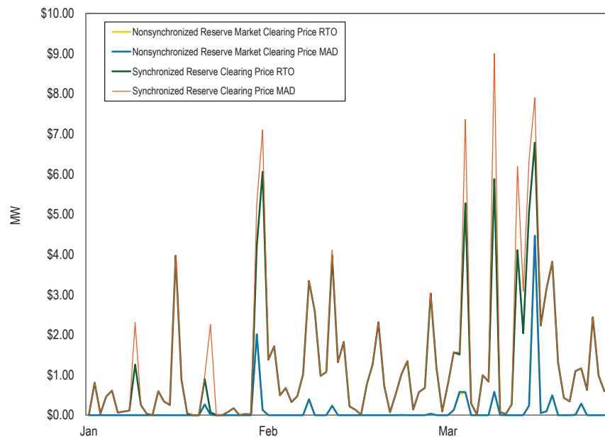
Figure 10-4 Daily average market clearing prices ($/MW) for synchronized reserve and nonsynchronized reserve: January through March 2019
