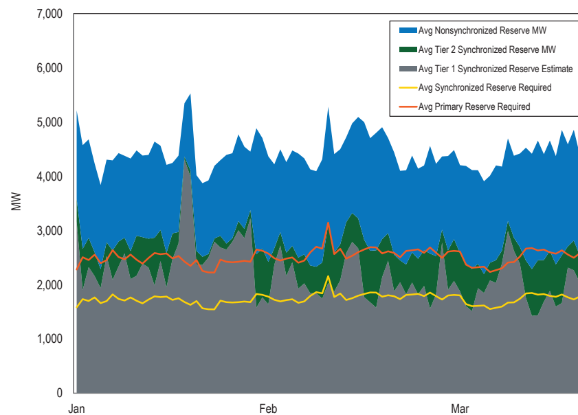
Figure 10-3 RTO reserve zone primary reserve MW by source (Daily Averages): January through March 2019
