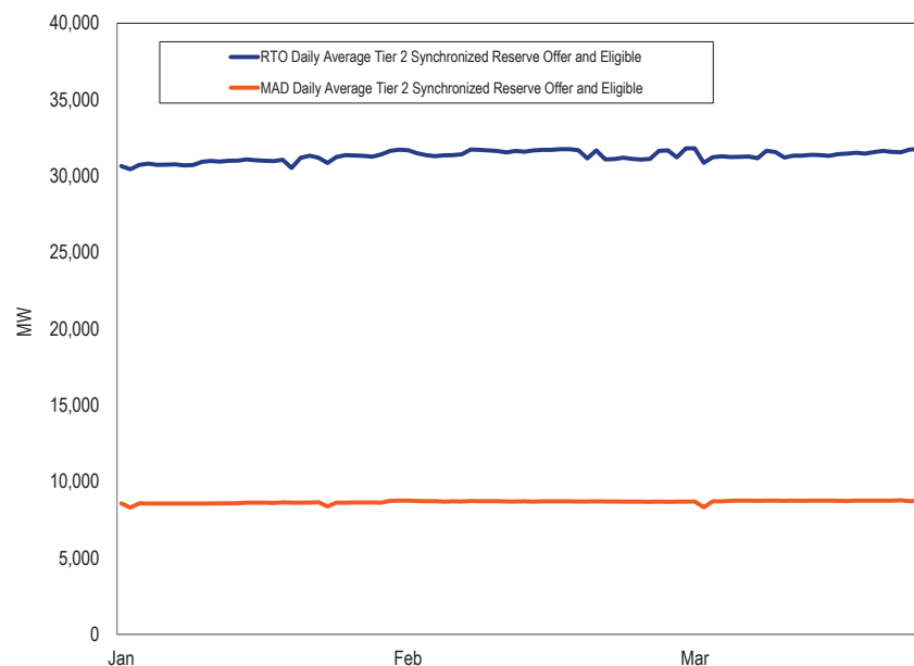
Figure 10-10 Tier 2 synchronized reserve hourly offer and eligible volume (MW): January through March, 2019
