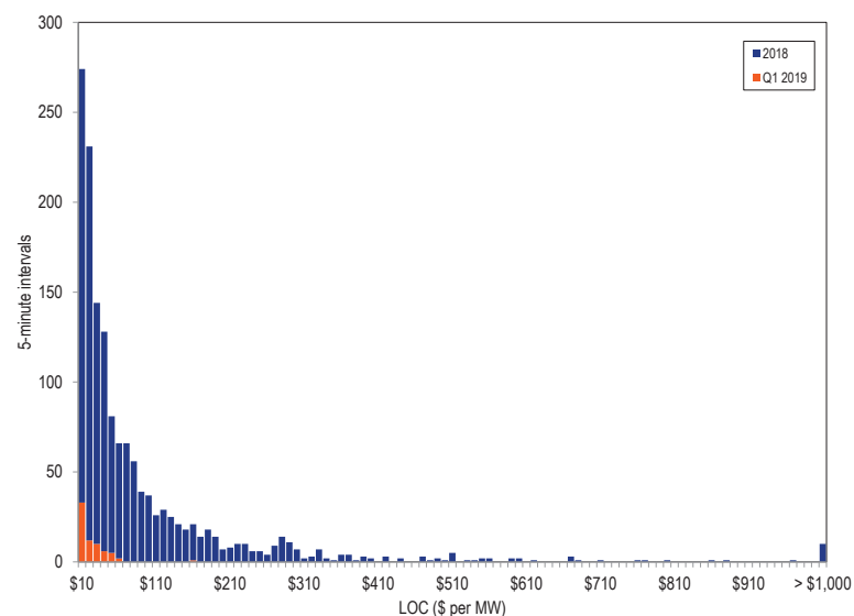
Figure 10-18 LOC distribution in each five-minute interval with a RegD marginal unit and an LOC greater than zero: January through March, 2019.
