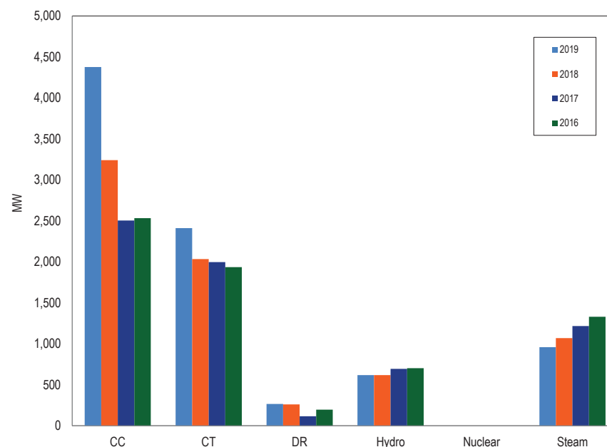
Figure 10-11 MAD average daily tier 2 synchronized reserve offer by unit type (MW): 2016 through 2019
