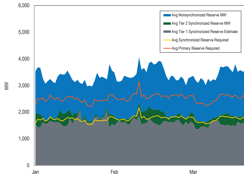
Figure 10-2 Mid-Atlantic Dominion subzone primary reserve MW by source (Daily Averages): January through March 2019
