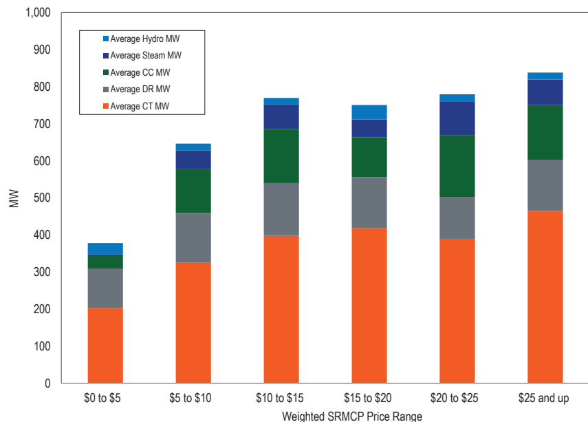
Figure 10-7 Average hourly tier 2 MW by unit type by weighted SRMCP range: January through March, 2019
