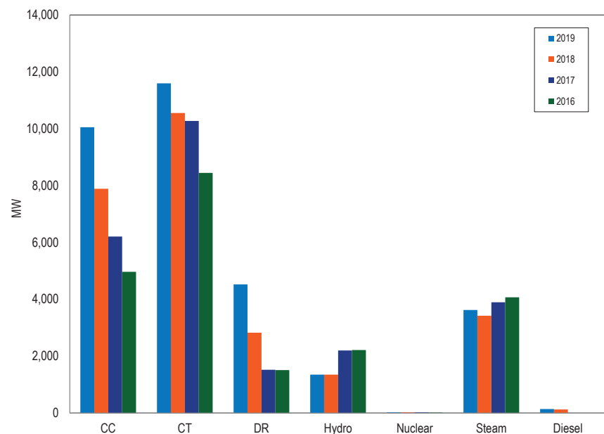
Figure 10-12 RTO Zone average daily tier 2 synchronized reserve offer by unit type (MW): January 2016 through March 2019
