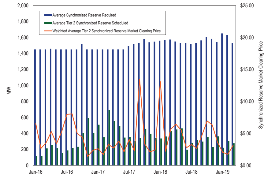
Figure 10-8 MAD hourly average tier 2 synchronized reserve scheduled MW: January 2016 through March 2019
