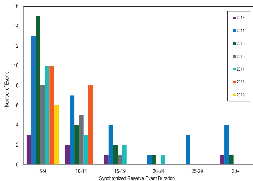
Figure 10-13 Synchronized reserve events duration distribution curve: January 2013 through March 2019
