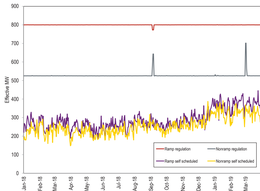
Figure 10-19 Nonramp and ramp regulation levels: January 2018 through March 2019 87
