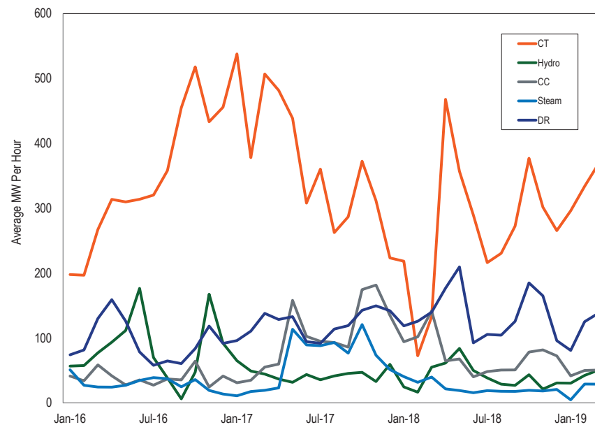
Figure 10-6 Cleared tier 2 synchronized reserve average MW per hour by unit type, RTO Zone: January 2016 through March 2019
