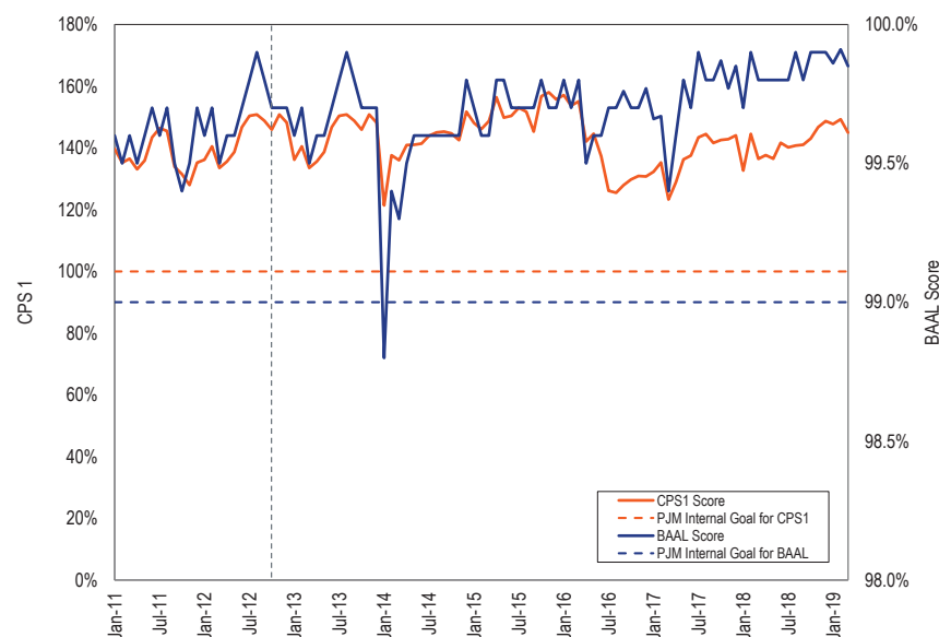
Figure 10-21 PJM monthly CPS1 and BAAL performance: January 2011 through March 2019
