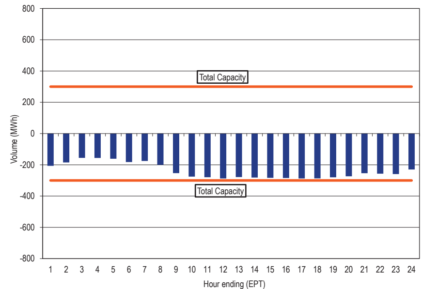
Figure 9-7 Linden hourly average flow: January through March, 2018 39
