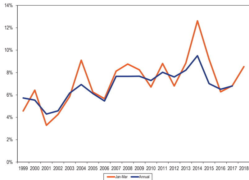
Figure 5-11 Trends in the PJM equivalent demand forced outage rate (EFORD): 1999 through 2018
