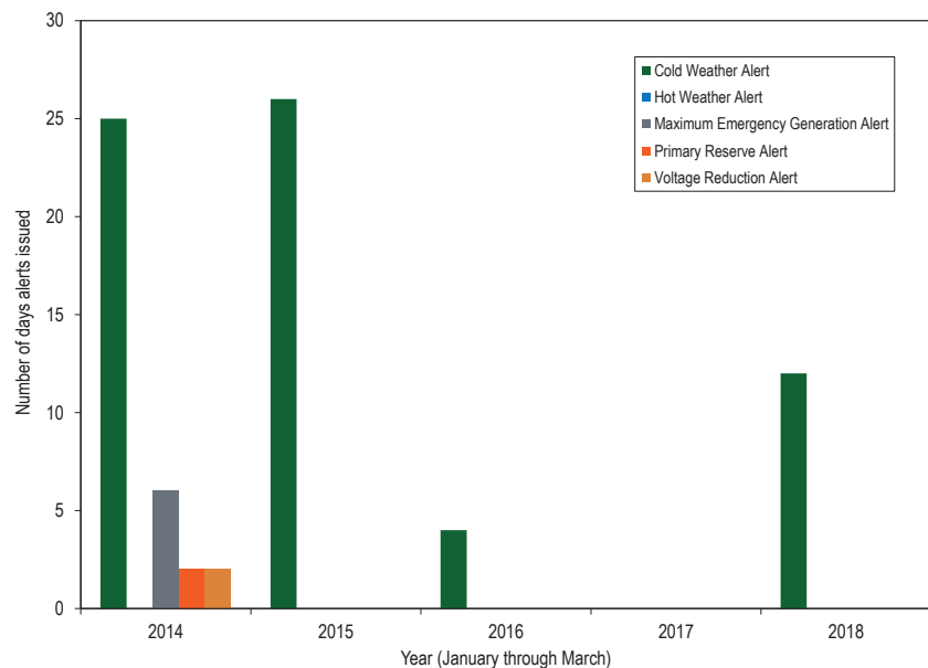
Figure 3-56 PJM declared emergency alerts: January through March, 2014 through 2018
