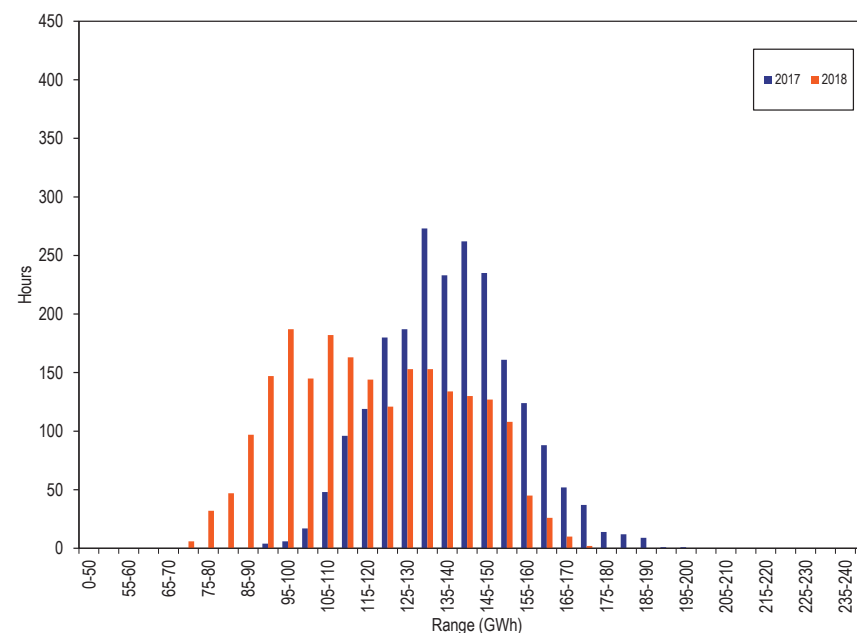
Figure 3-21 Distribution of PJM day-ahead demand plus exports: January through March, 2017 and 2018 42
