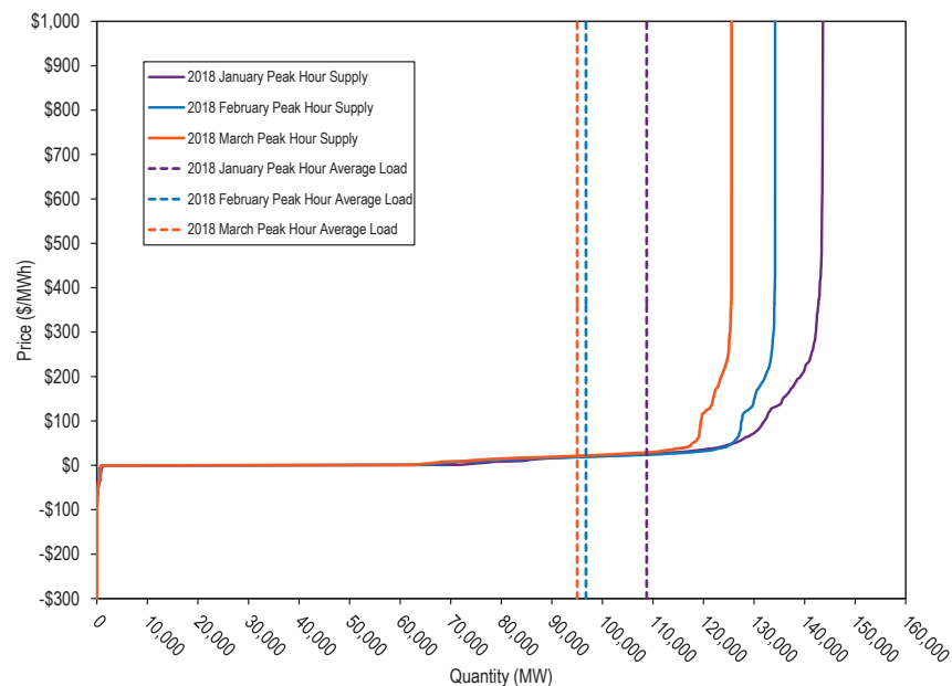
Figure 3-6 Average hourly real time supply curves: January through March, 2018
