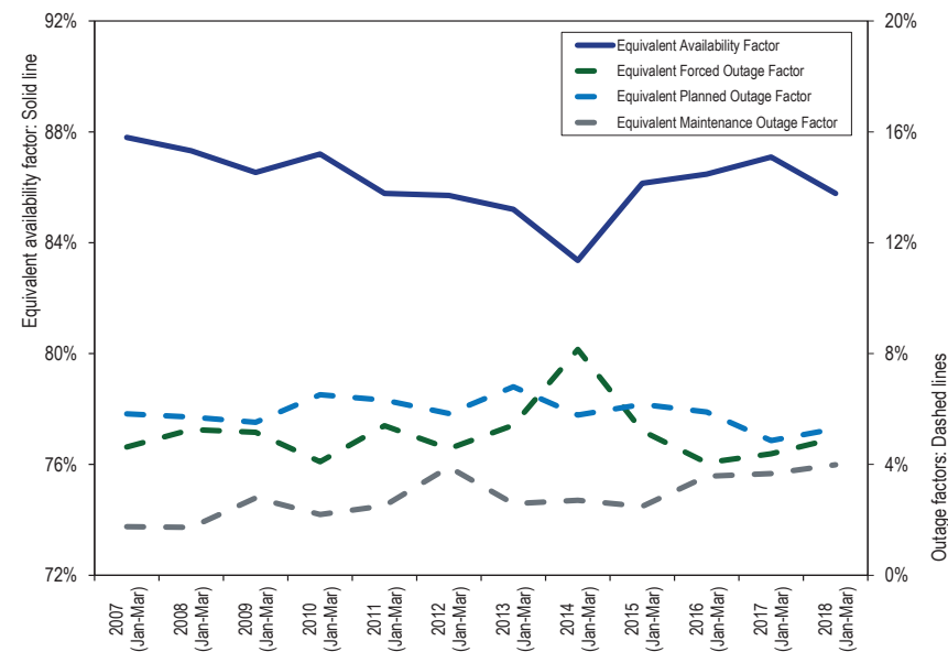
Figure 5-10 PJM equivalent outage and availability factors: January through March, 2007 to 2018
