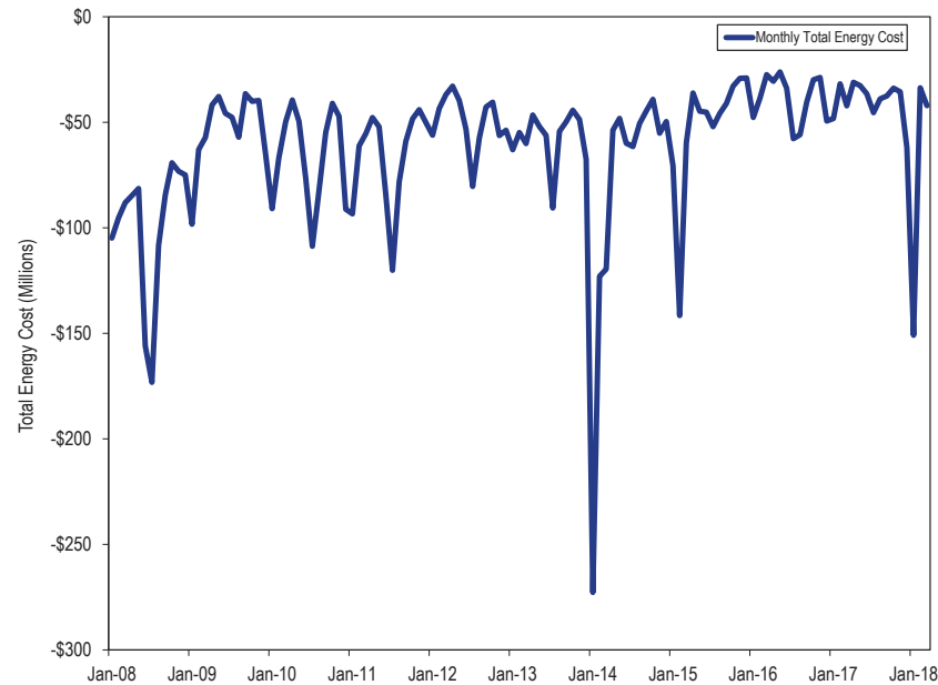
Figure 11-8 PJM monthly energy costs (Millions): January 2008 through March 2018
