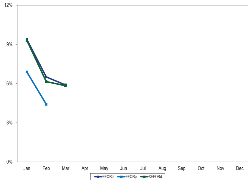
Figure 5-12 PJM EFORd, XEFORd and EFORp: January through March, 2018
