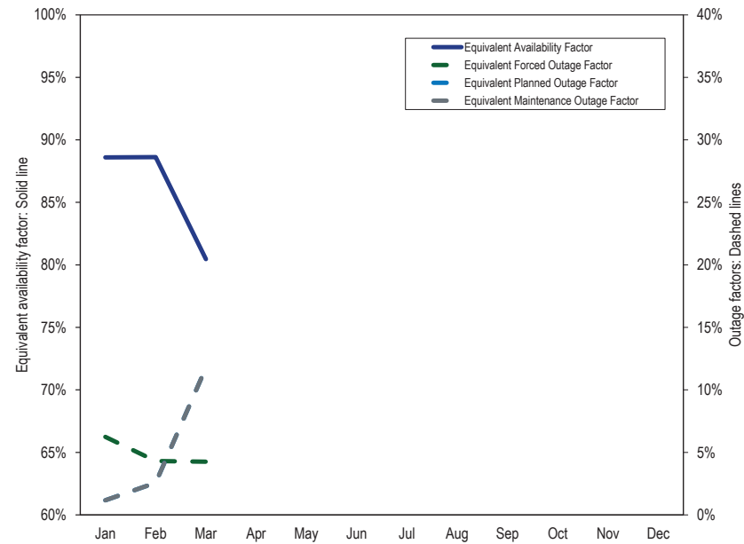
Figure 5-13 PJM monthly generator performance factors: January through March, 2018
