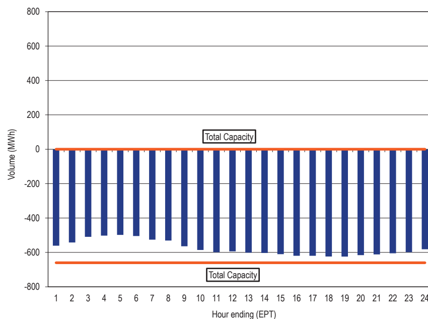
Figure 9-8 Hudson hourly average flow: January through March, 2018
