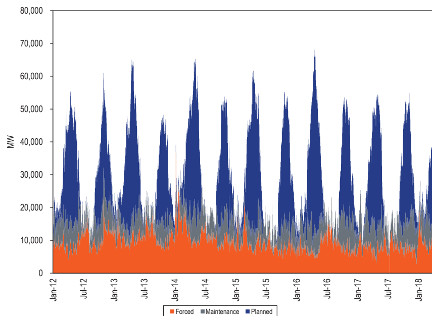
Figure 5-9 PJM outages (MW): 2012 through March 2018
