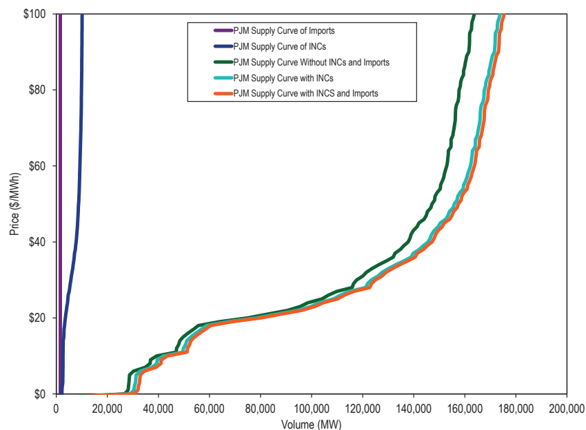
Figure 3-35 Typical dispatch price range for PJM day-ahead aggregate supply curves: 2017 example day
