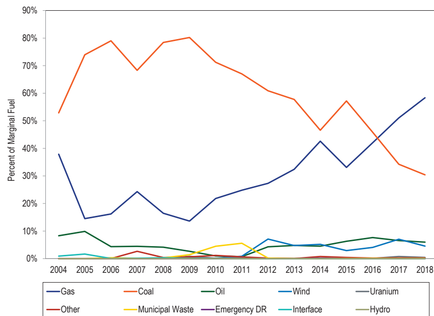
Figure 3-4 Type of fuel used (By real-time marginal units): January through March, 2004 through 2018
