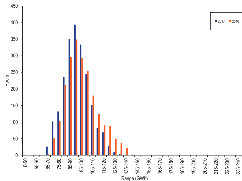
Figure 3-9 Distribution of PJM real-time generation plus imports: January through March, 2017 and 2018 30
