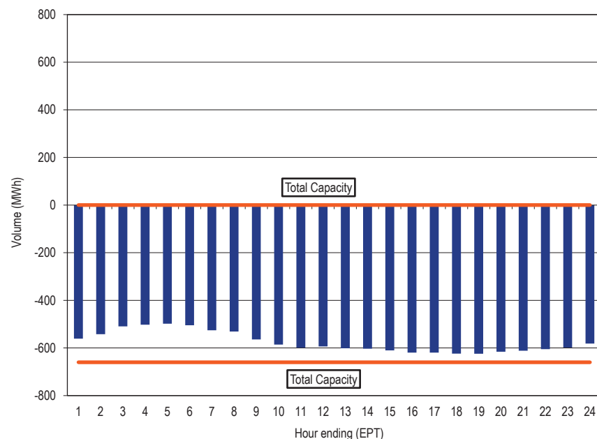
Figure 9-6 Neptune hourly average flow: January through March, 2018
