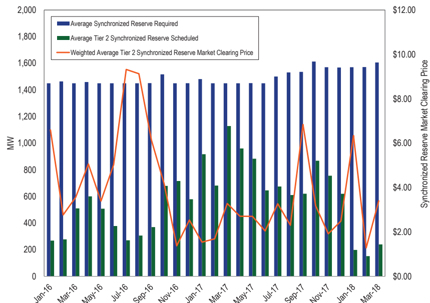
Figure 10-9 RTO monthly average tier 2 synchronized reserve scheduled MW: January 2016 through March 2018
