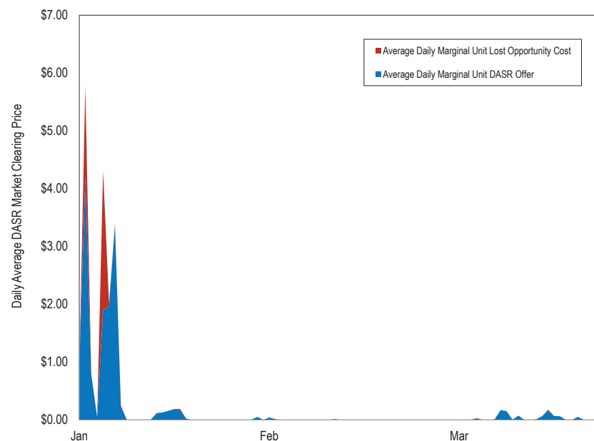
Figure 10-15 Daily average components of DASR clearing price ($/MW), marginal unit offer and LOC: January through March 2018
