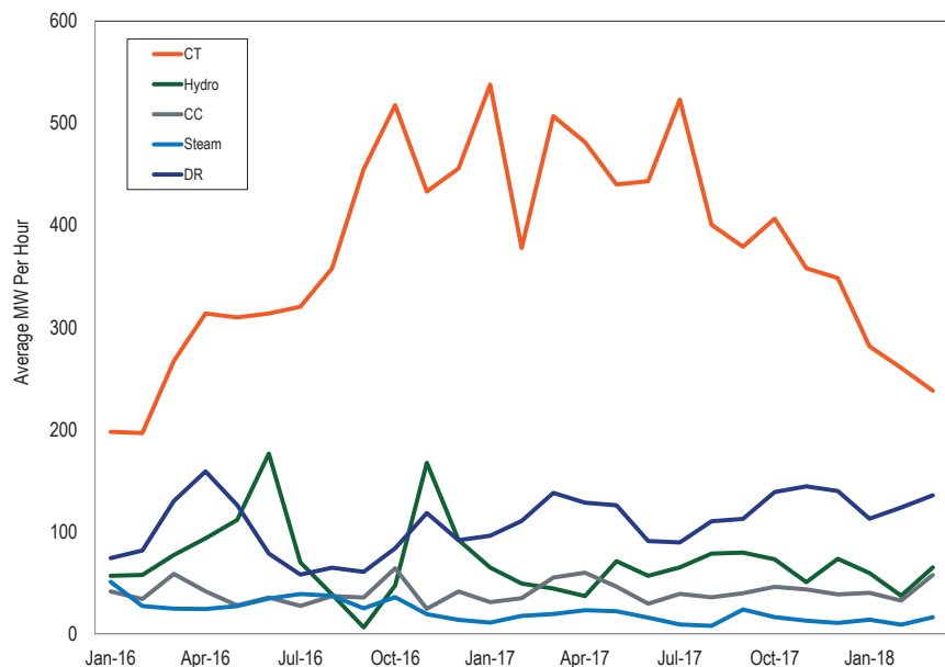
Figure 10-6 Cleared tier 2 synchronized reserve average hourly MW per hour by unit type, RTO Zone: January 2016 through March 2018
