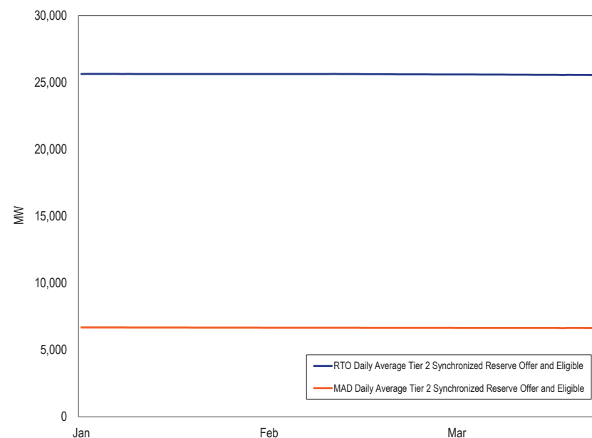
Figure 10-10 Tier 2 synchronized reserve hourly offer and eligible volume (MW), averaged daily: January through March, 2018
