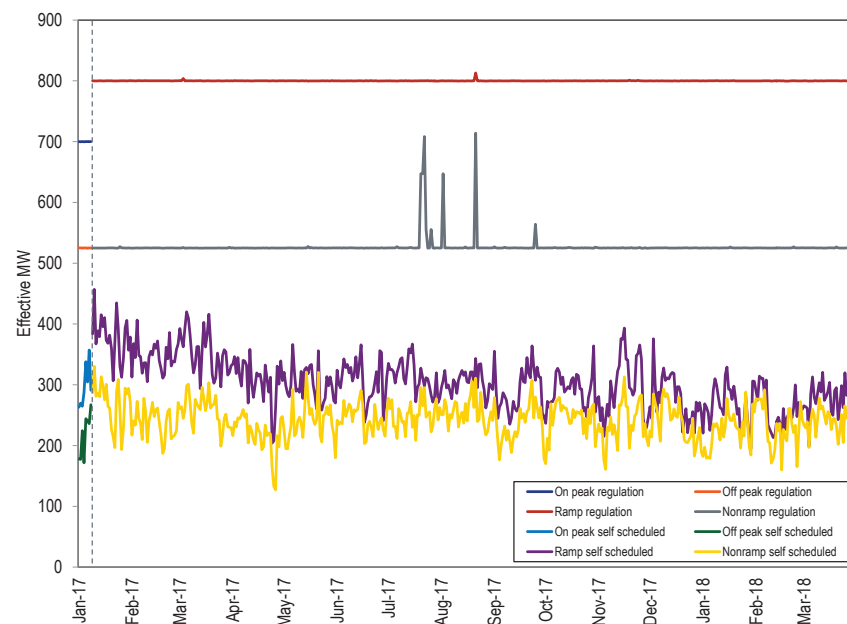
Figure 10-26 Off peak, on peak, nonramp, and ramp regulation levels: January 2017 through March 2018 80
