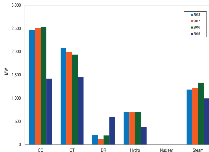
Figure 10-11 MAD average daily tier 2 synchronized reserve offer by unit type (MW): January 2015 through March 2018
