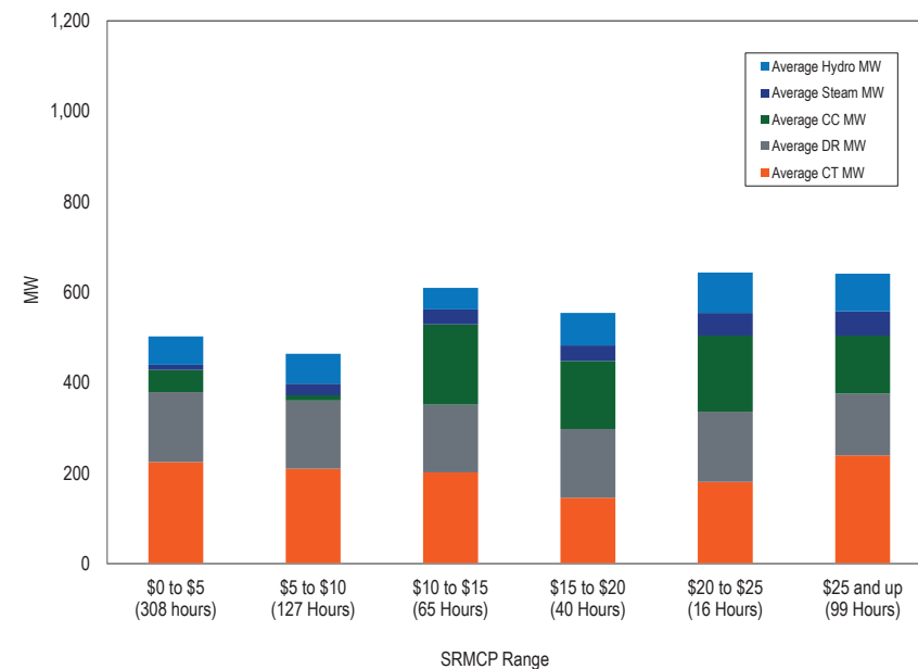
Figure 10-7 Average hourly tier 2 MW by unit type by SRMCP range: January through March, 2018
