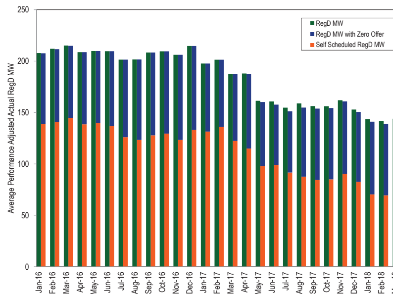
Figure 10-24 Average cleared RegD MW and average cleared RegD with an effective price of $0.00 by month: January 2016 through March 2018
