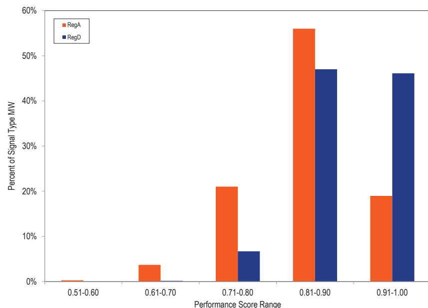
Figure 10-17 Hourly average performance score by regulation signal type: January through March, 2018
