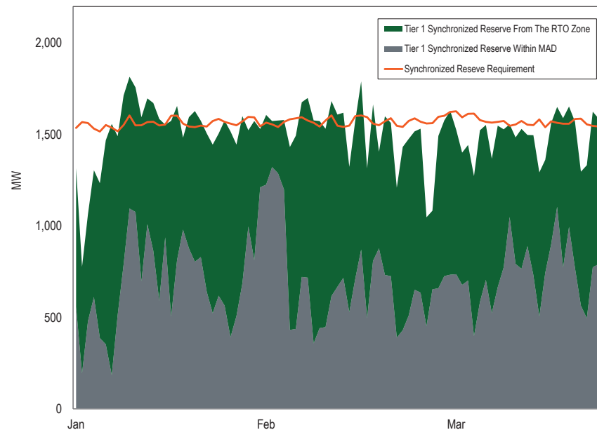
Figure 10-5 Daily average tier 1 synchronized reserve supply (MW) in the MAD Subzone: January through March, 2018
