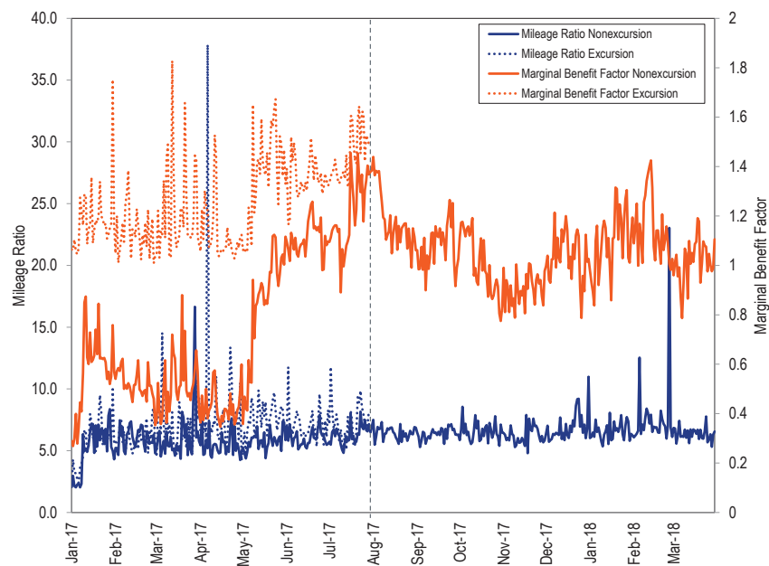
Figure 10-18 Daily average MBF and mileage ratio during excursion and nonexcursion hours: January 2017 through March 2018 63
