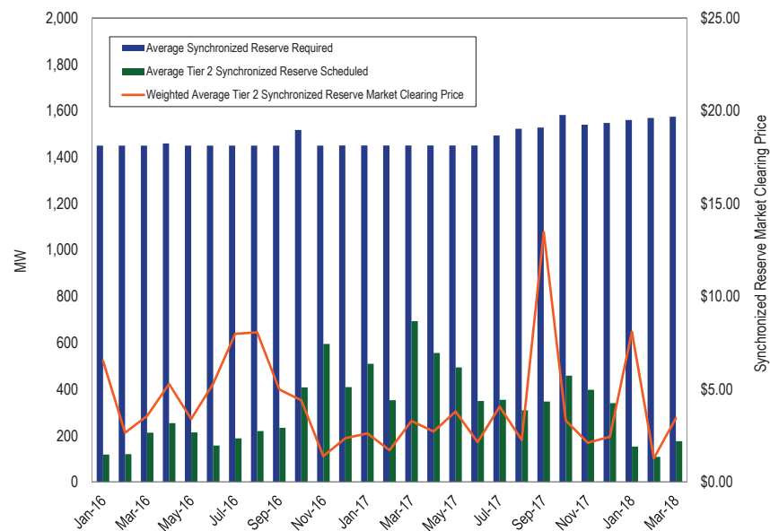
Figure 10-8 MAD monthly average tier 2 synchronized reserve scheduled MW: January 2016 through March 2018
