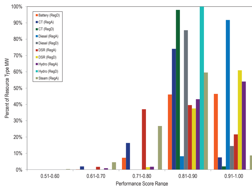
Figure 10-16 Hourly average performance score by unit type: January through March, 2018
