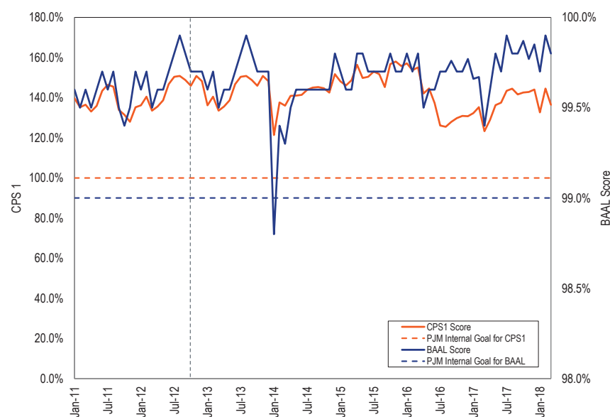
Figure 10–28 PJM monthly CPS1 and BAAL performance: January 2011 through March 2018
