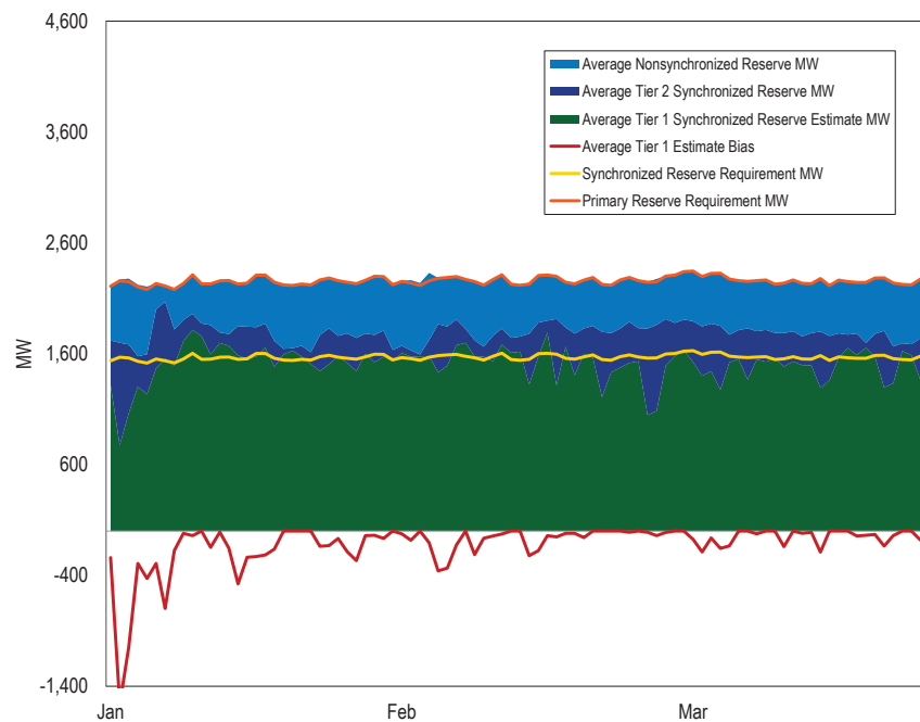
Figure 10-2 Mid-Atlantic Dominion subzone primary reserve MW by source (Daily Averages): January through March, 2018
