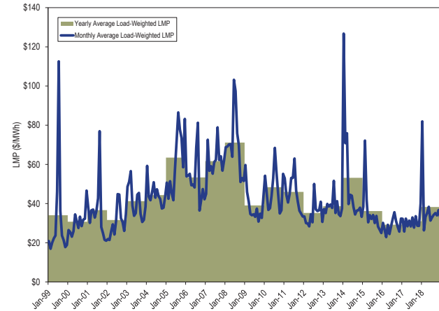
Figure 8 Real-time, monthly and annual, load-weighted, average LMP: January 1999 through December 2018
