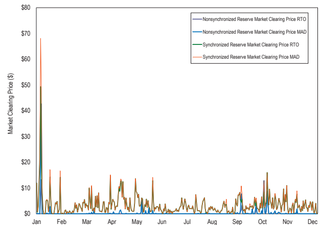
Figure 18 Daily average market clearing prices ($/MW) for synchronized reserve and nonsynchronized reserve: 2018
