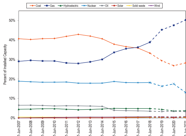
Figure 10 Percent of installed capacity (By fuel source): June 1, 2007 through June 1, 2021
