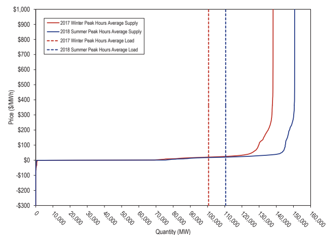
Figure 7 Average hourly real-time supply curves: 2017 winter and 2018 summer 69
