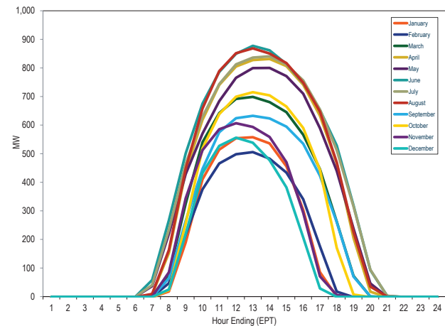
Figure 16 Average hourly real-time generation of solar units in PJM: 2018
