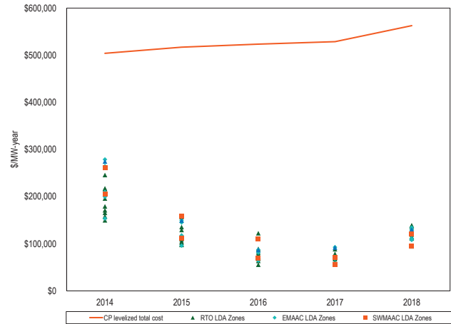
Figure 14 New entrant CP net revenue and 20-year leveled total cost by LDA (Dollars per installed MW-year): 2014 through 2018
