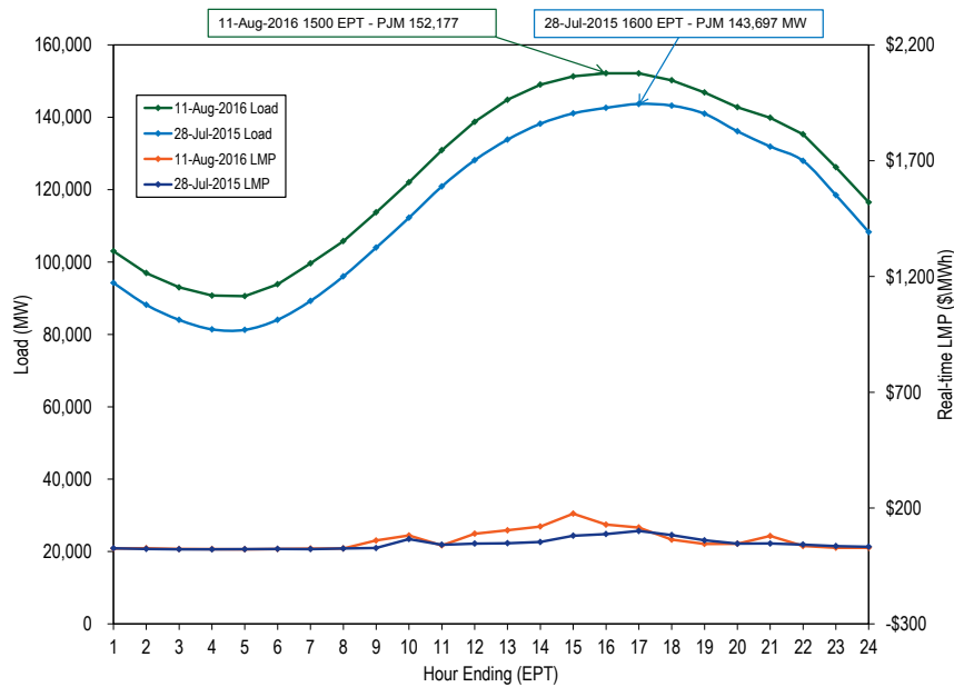
Figure 3-14 PJM peak-load comparison Thursday, August 11, 2016 and Tuesday, July 28, 2015
