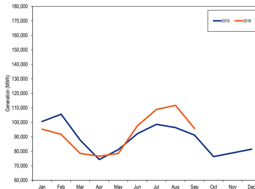
Figure 3-7 PJM real-time average monthly hourly generation: 2015 through September 2016
