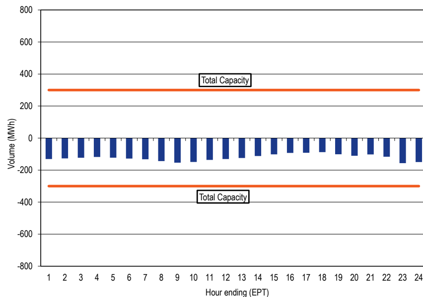
Figure 9–7 Linden hourly average flow: January through September, 2016 41
