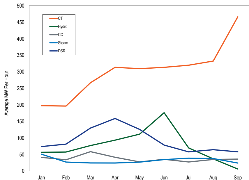
Figure 10-7 Cleared tier 2 synchronized reserve average hourly MW per hour by unit type, RTO Zone: January through September, 2016
