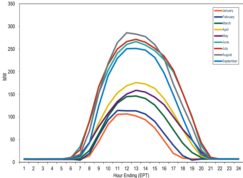
Figure 8-13 Average hourly day-ahead generation of solar units in PJM: January through September 2016
