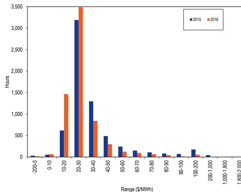
Figure 3-36 Average LMP for the PJM Real-Time Energy Market: January through September, 2015 and 2016
