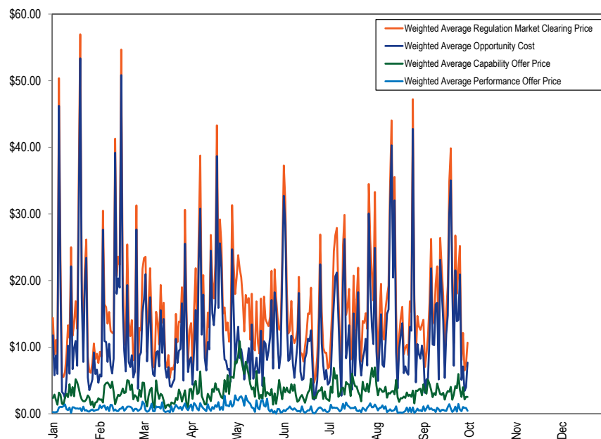
Figure 10–31 PJM regulation market daily weighted average market-clearing price, marginal unit opportunity cost and offer price (Dollars per MW): January through September, 2016
