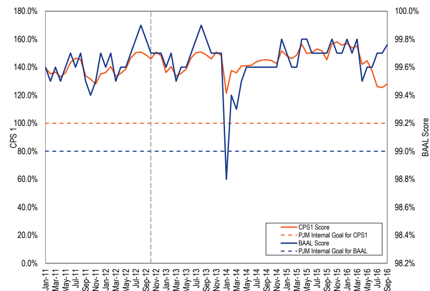
Figure 10-32 PJM monthly CPS1 and BAAL performance: January 2011 through September 2016
