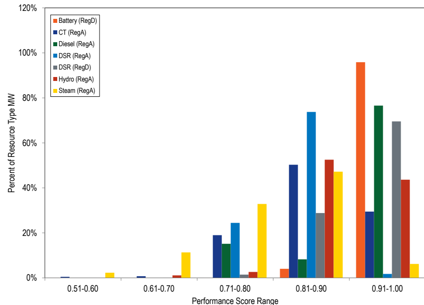
Figure 10-19 Hourly average performance score by unit type: January through September, 2016
