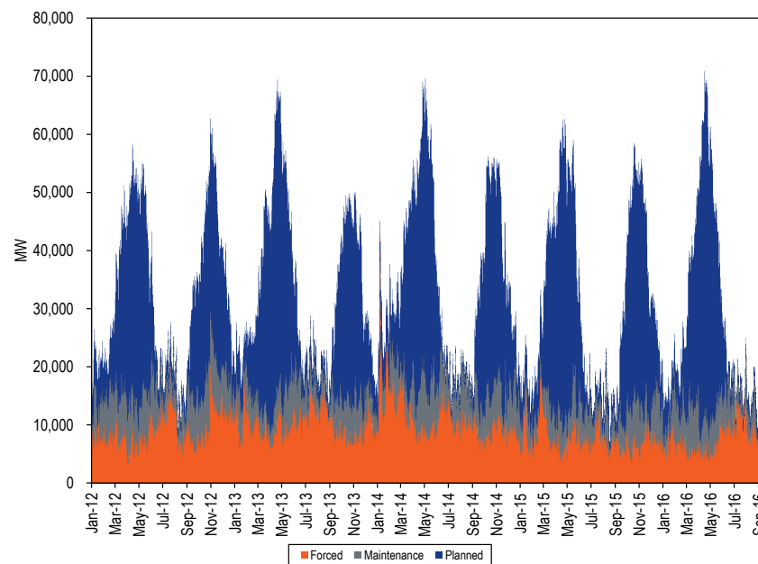
Figure 5-8 PJM outages (MW): 2012 through September 2016
