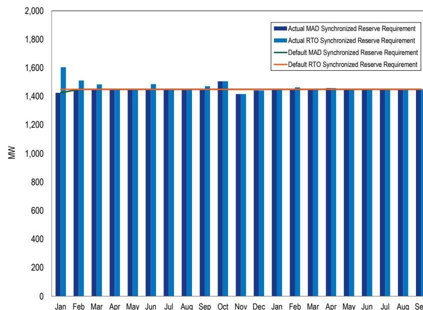
Figure 10–9 Monthly average actual vs default synchronized reserve requirements, RTO Zone and MAD Subzone: January 2015 through September 2016
