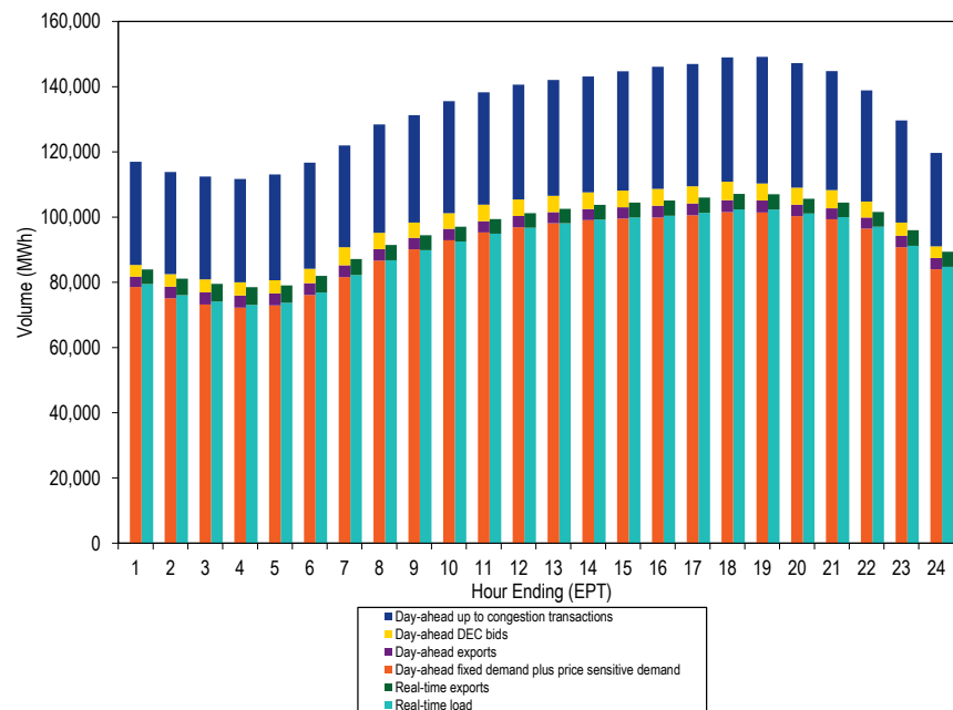
Figure 3-20 Day-ahead and real-time demand (Average hourly volumes): January through September, 2016
