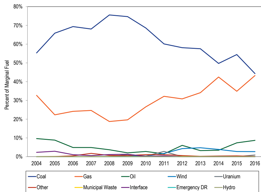
Figure 3-3 Type of fuel used (By real-time marginal units): January through September, 2004 through 2016
