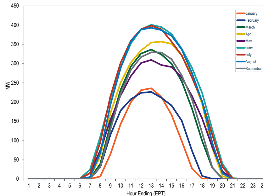
Figure 8-12 Average hourly real-time generation of solar units in PJM: January through September 2016
