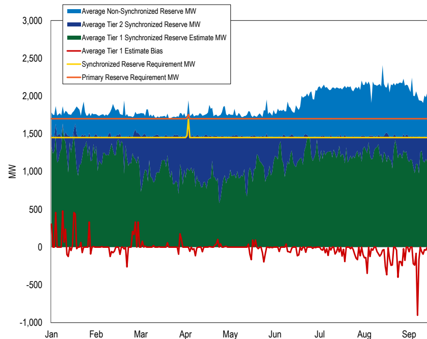
Figure 10-2 Mid-Atlantic Dominion Subzone primary reserve MW by source (Daily Averages): January through September, 2016
