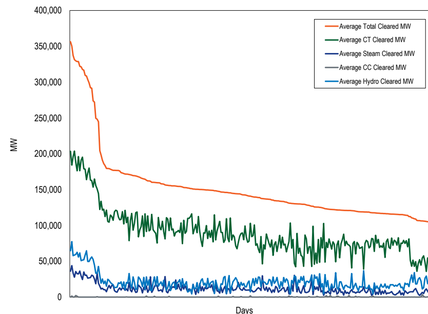
Figure 10-18 Daily average DASR MW by unit type sorted from highest to lowest daily requirement: January through September, 2016
