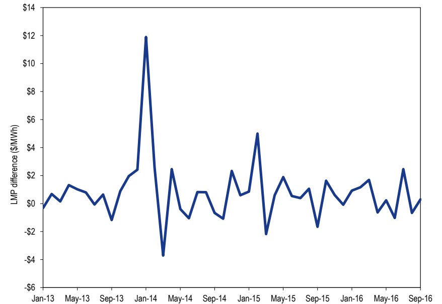
Figure 3-47 Monthly average of real-time minus day-ahead LMP: January 2013 through September 2016
