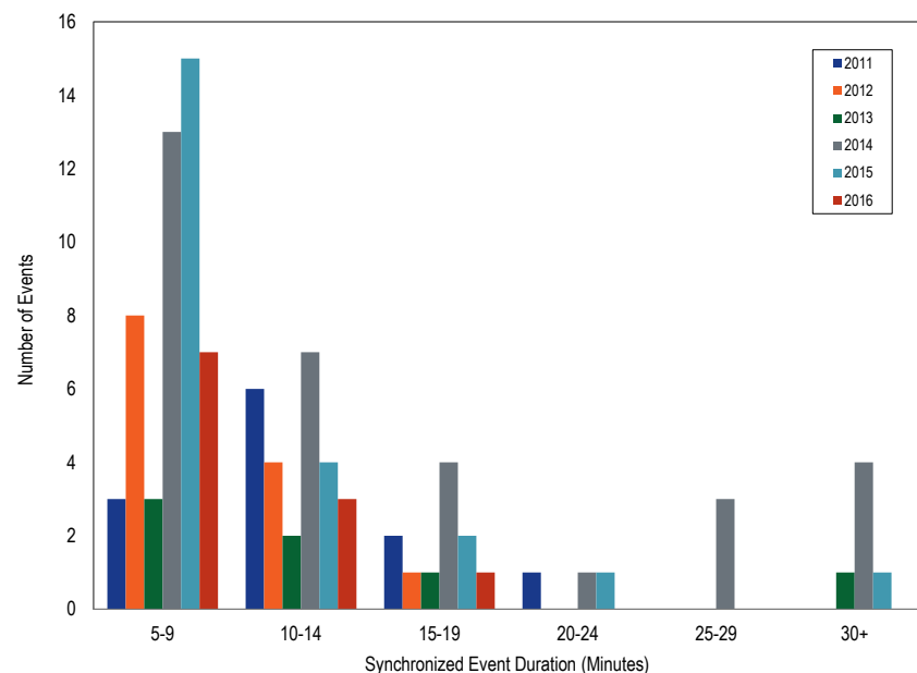
Figure 10-15 Synchronized reserve events duration distribution curve: 2011 through 2016
