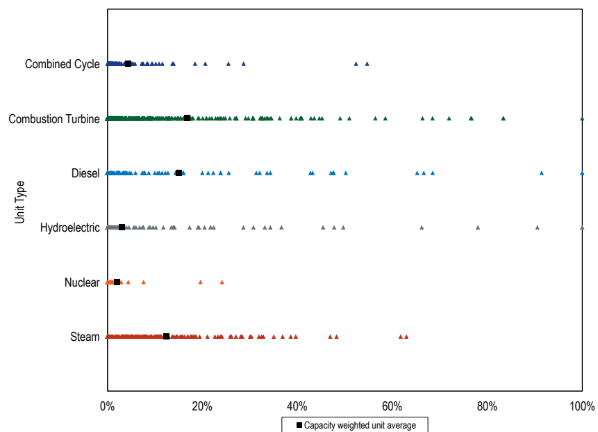
Figure 5-11 PJM distribution of EFORd data by unit type: January through September, 2016
