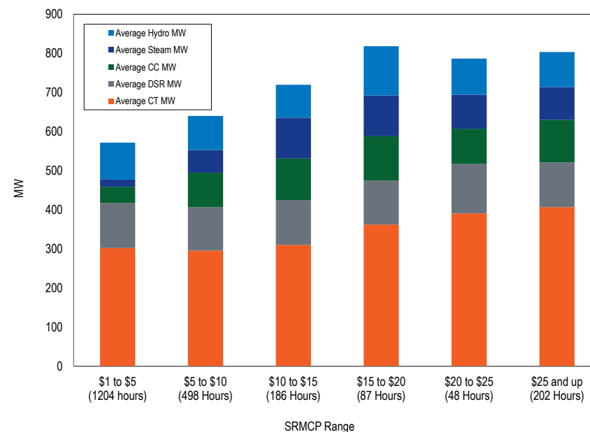
Figure 10-8 Average hourly tier 2 MW by unit type by SRMCP range: January through September, 2016
