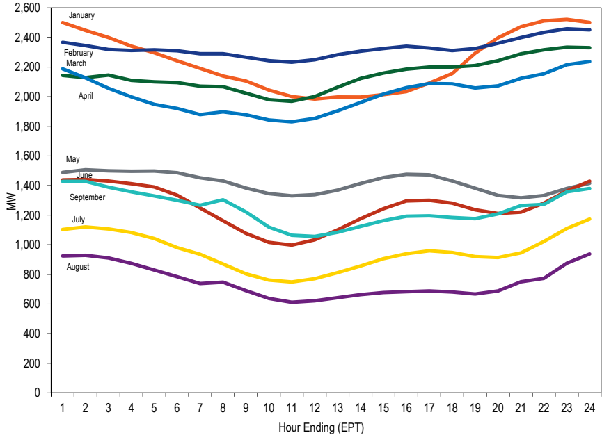
Figure 8-10 Average hourly day-ahead generation of wind units in PJM: January through September 2016
