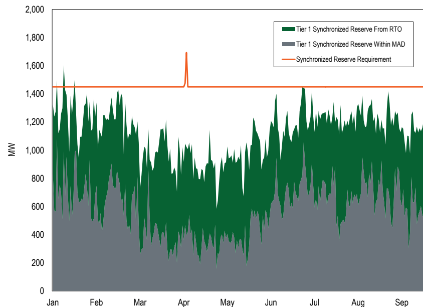
Figure 10-5 Daily average tier 1 synchronized reserve supply (MW) in the MAD Subzone: January through September, 2016
