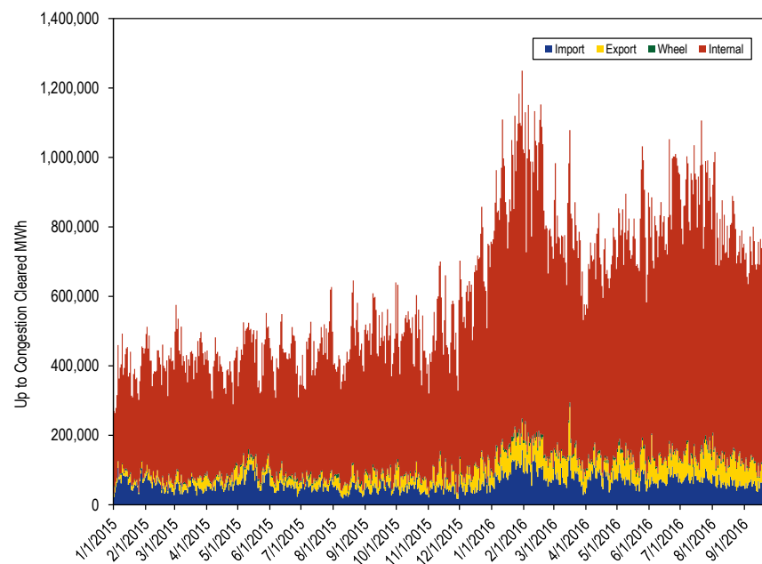
Figure 3-33 PJM daily cleared up to congestion transaction by type (MW): January 2015 through September 2016
