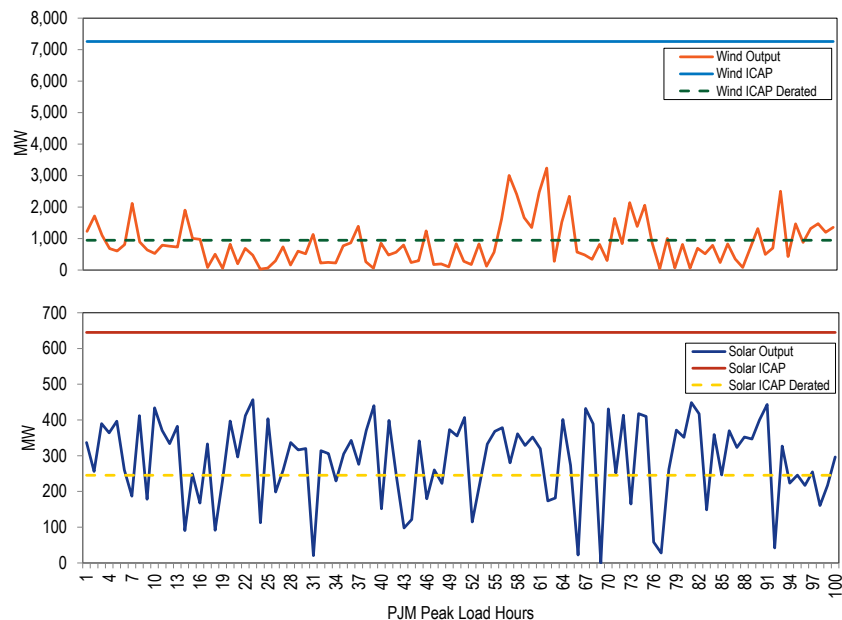
Figure 8-8 Wind and solar output during the top 100 peak load hours in PJM: January through September 2016
