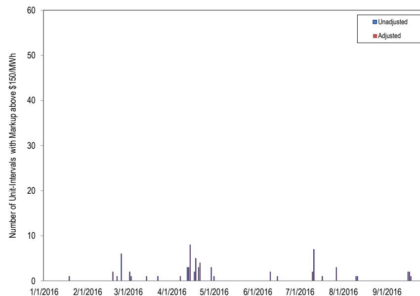
Figure 3-26 Number of Unit Intervals with markups above $150 per MWh: January through September, 2016
