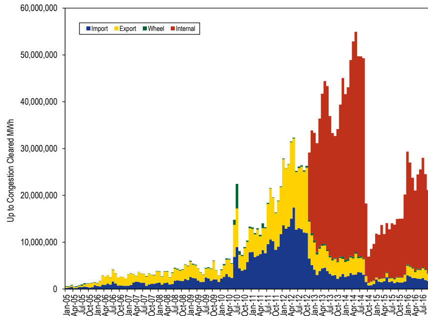
Figure 3-32 PJM monthly cleared up to congestion transactions by type (MWh): January 2005 through September 2016
