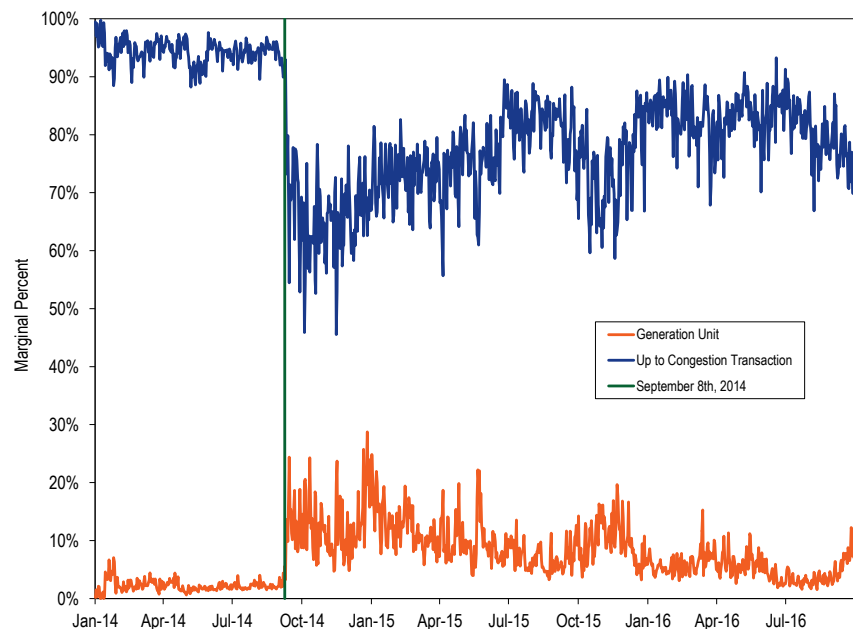
Figure 3-4 Day-ahead marginal up to congestion transaction and generation units: 2014 through September of 2016
