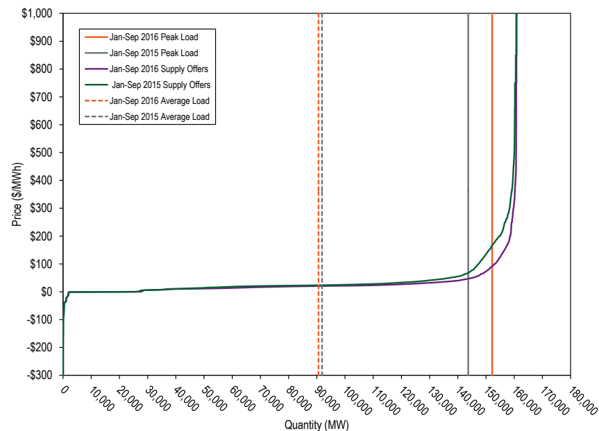
Figure 3-5 Average PJM aggregate real-time generation supply curves by offer price: January through September, 2015 and 2016
