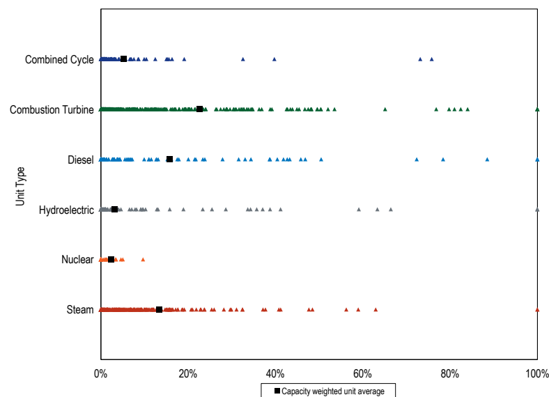
Figure 5-11 PJM distribution of EFORD data by unit type: January through June, 2016
