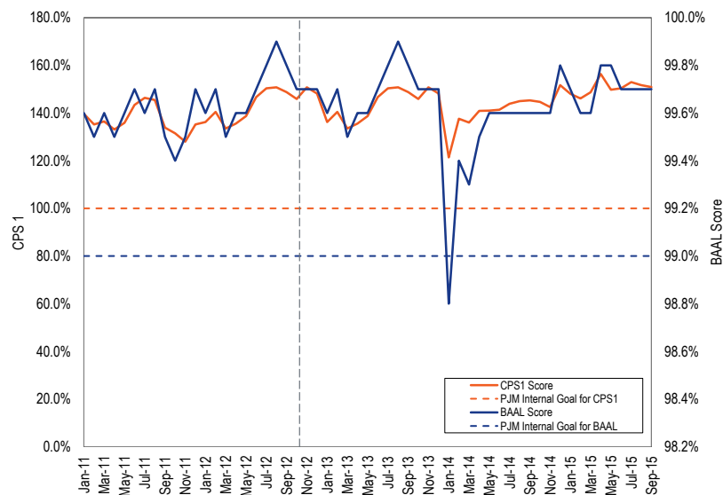
Figure 10-28 PJM monthly CPS1 and BAAL performance: January 2011 through September 2015
