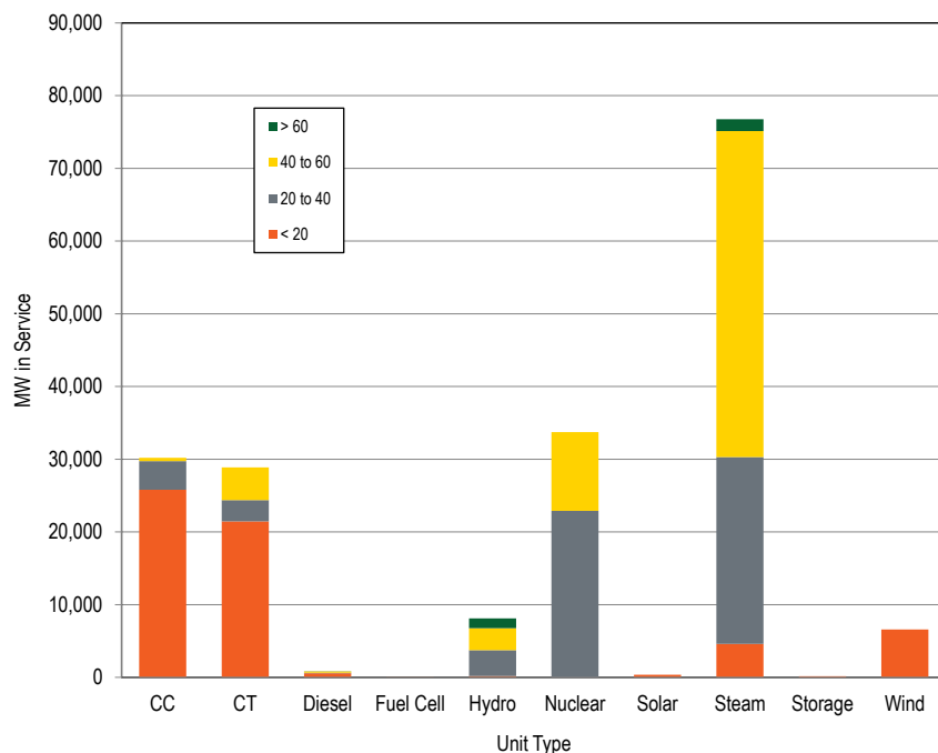
Figure 12-2 PJM capacity (MW) by age (years): At September 30, 2015
