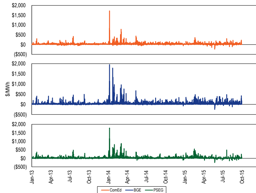
Figure 7-4 Dark spread for selected zones: 2013 through 2015 19
