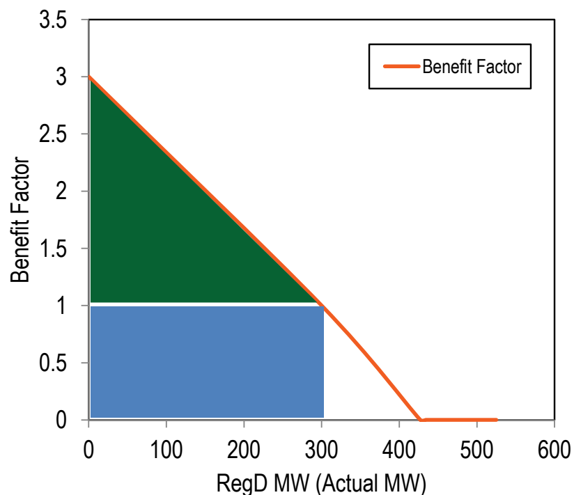
Figure 10-24 Illustration of correct method for calculating effective MW
