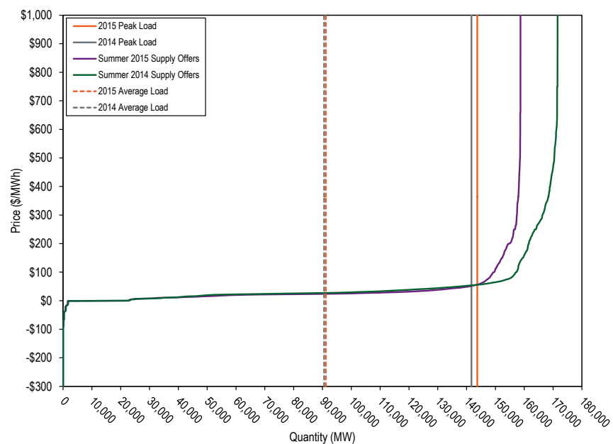
Figure 3-4 Average PJM aggregate real-time generation supply curves by offer price: Summer of 2014 and 2015
