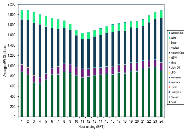
Figure 8-9 Marginal fuel at time of wind generation in PJM: 2015
