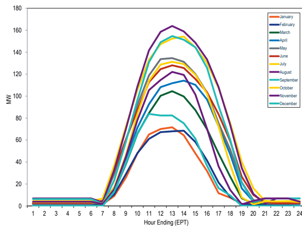
Figure 8-11 Average hourly day-ahead generation of solar units in PJM: 2015
