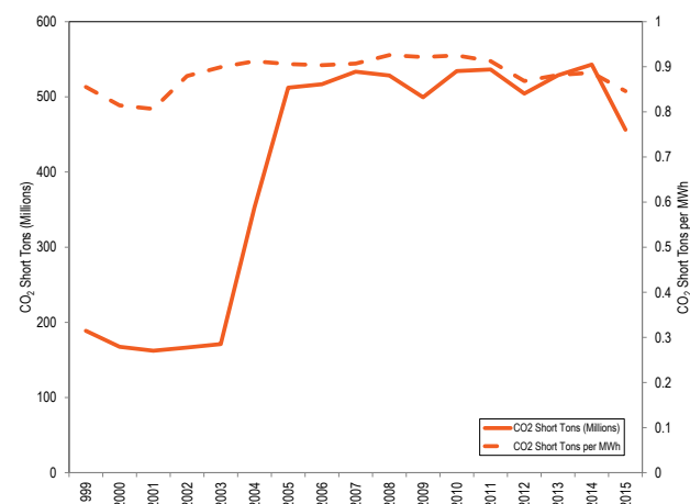
Figure 8-5 CO 2 emissions by year (millions of short tons), by PJM units: 1999 through 2015 132
