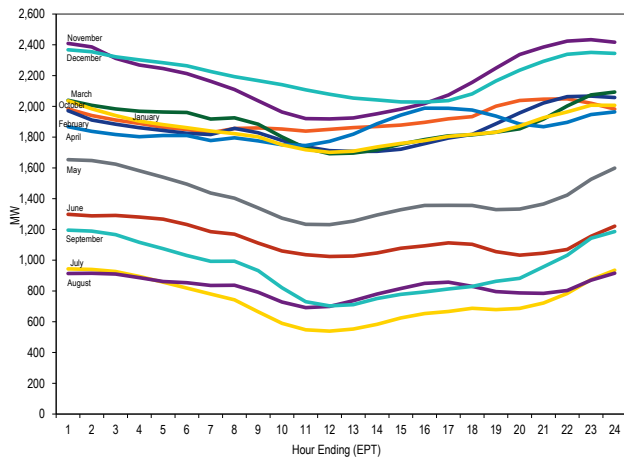
Figure 8-8 Average hourly day-ahead generation of wind units in PJM: 2015
