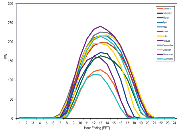
Figure 8-10 Average hourly real-time generation of solar units in PJM: 2015
