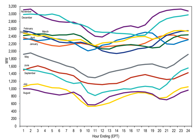
Figure 8-7 Average hourly real-time generation of wind units in PJM: 2015
