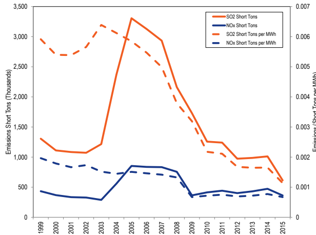
Figure 8-6 SO 2 and NO x emissions by year (thousands of short tons), by PJM units: 1999 through 2015 133
