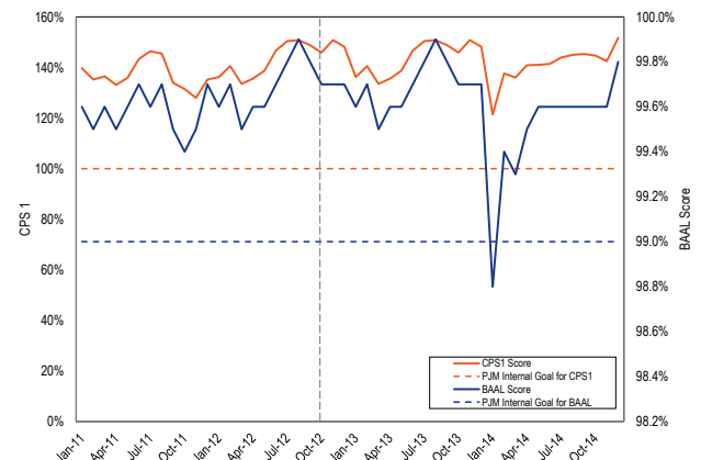
Figure F-3 PJM CPS1/BAAL performance: 2014
