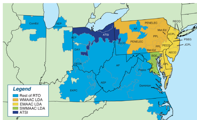
Figure A-3 PJM locational deliverability areas
