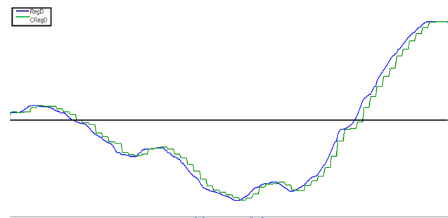
Figure F-6 PJM RegD signal and CRegD compliance signal. Screenshot of typical 10-minute time period
