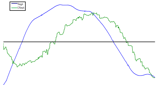
Figure F-5 PJM RegA signal and CRegA compliance signal. Screenshot of typical 10-minute time period
