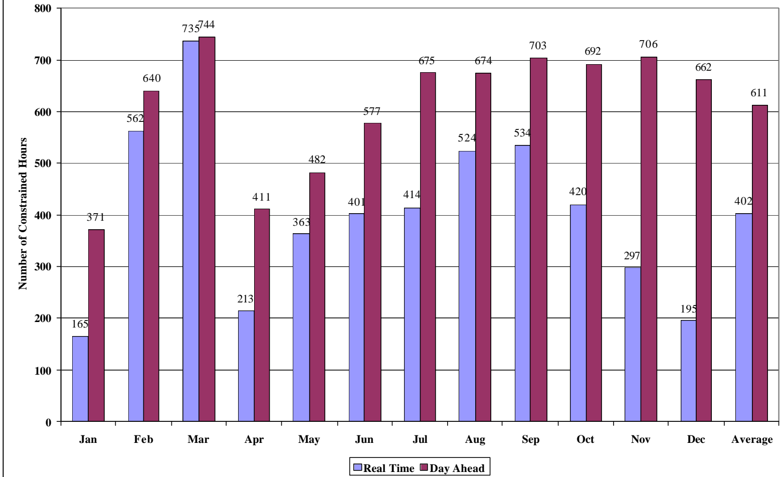
Figure A.14: Real Time and Day Ahead Market Constrained Hours - 2001
