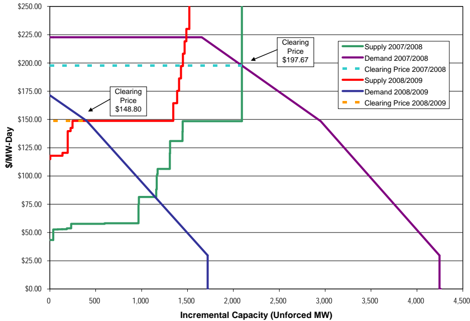
Figure 8 EMAAC incremental supply/demand curves: 2007-2008 and 2008-2009 RPM auctions 47, 48
