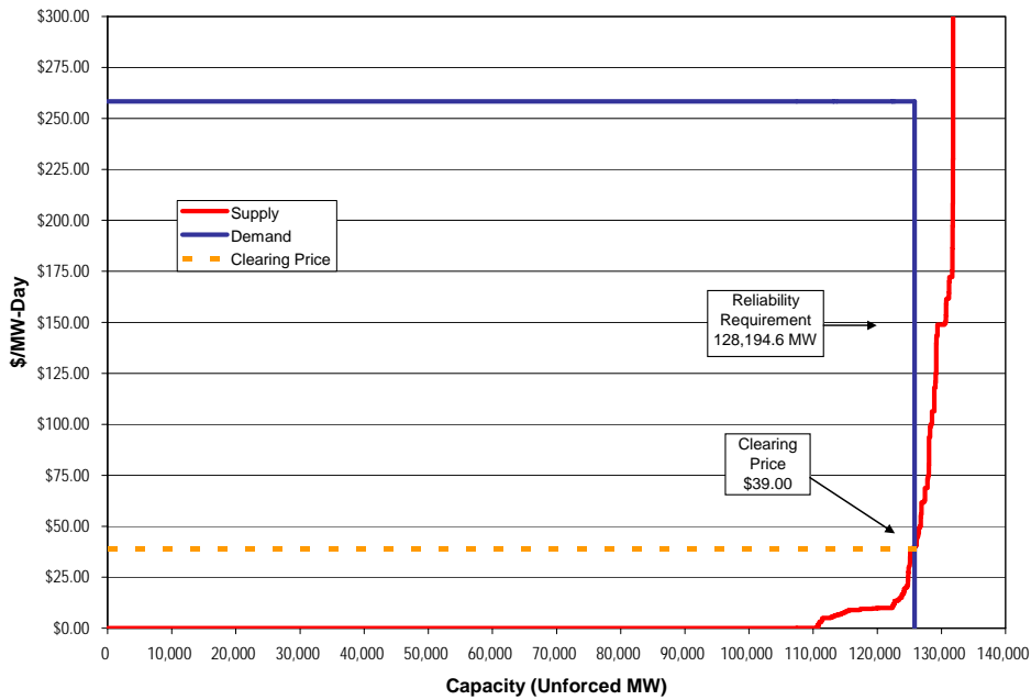
Figure 2 PJM RTO supply/demand curves at reliability requirement: 2008-2009 RPM auction 32, 33, 34
