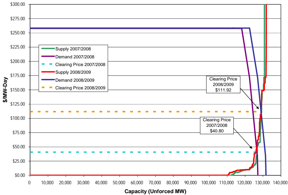
Figure 3 RTO market supply/demand curves: 2007-2008 and 2008-2009 RPM auctions 35, 36
