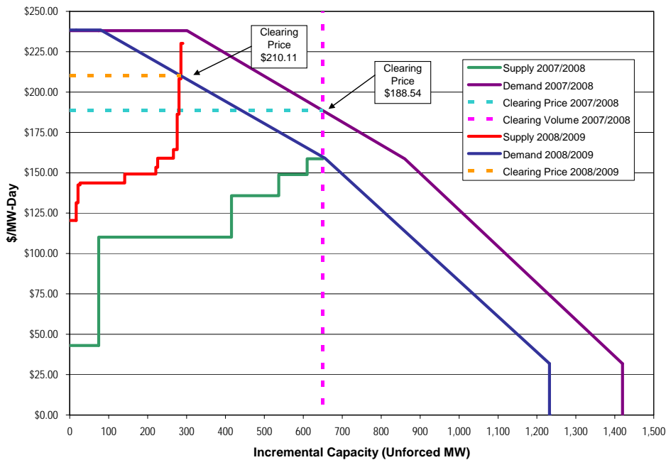
Figure 11 SWMMAC incremental supply/demand curves: 2007-2008 and 2008-2009 RPM auctions 53, 54
