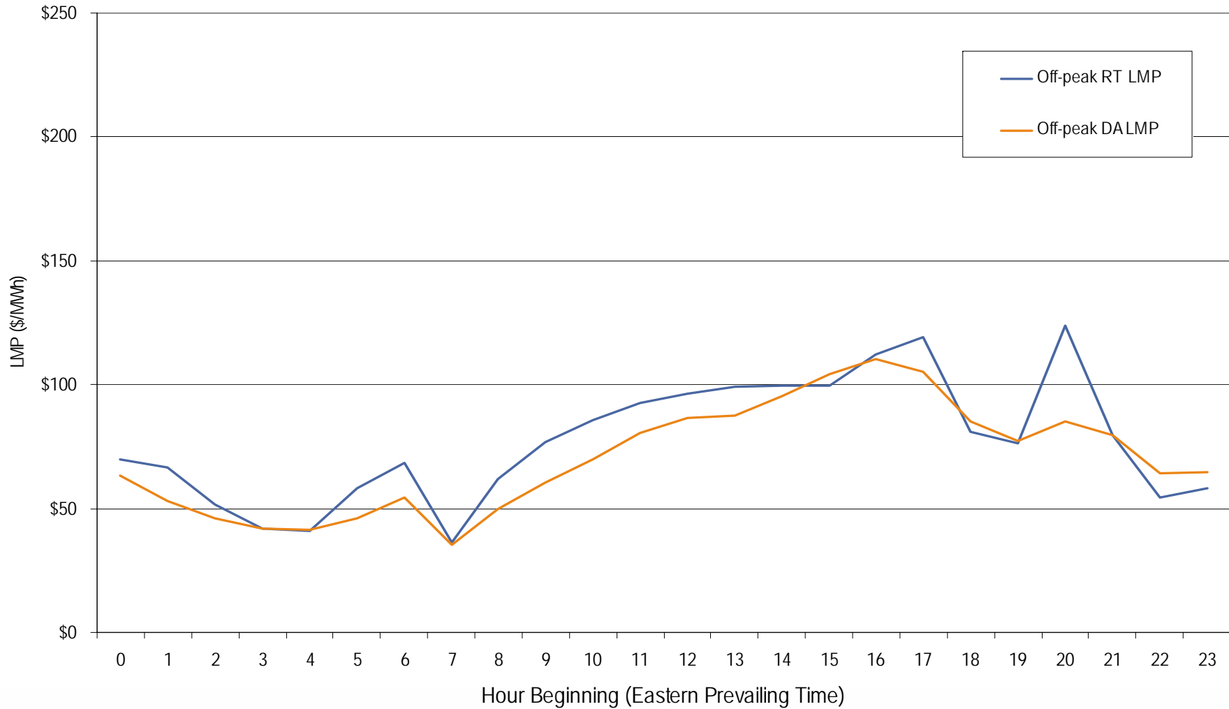
Dominion real-time and day-ahead hourly average off-peak LMP August 2006
