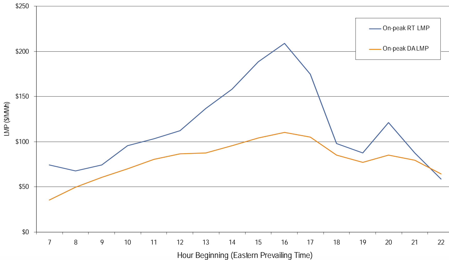
Dominion real-time and day-ahead hourly average on-peak LMP August 2006
