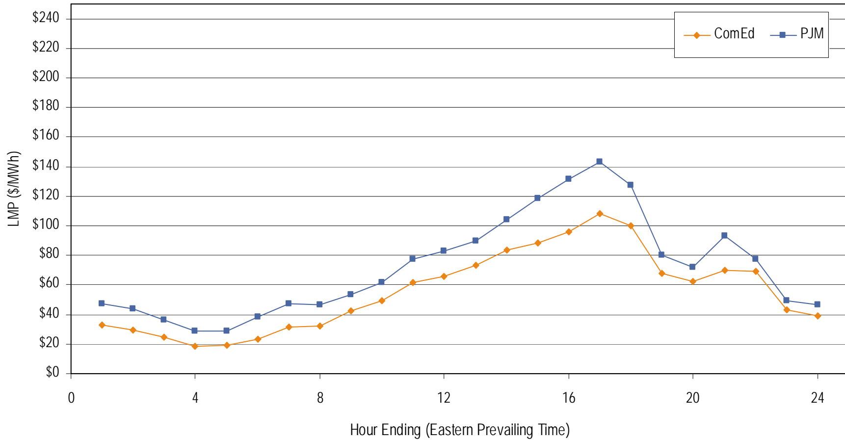
Average Hourly Real-Time LMP August 2006
