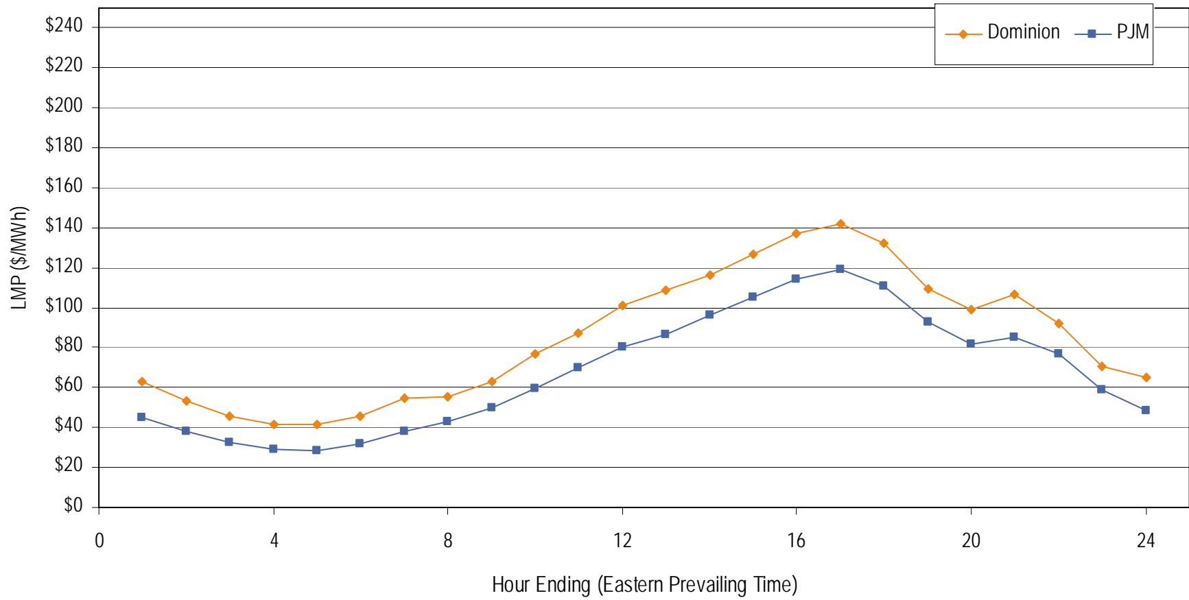
Average Hourly Day-Ahead LMP August 2006
