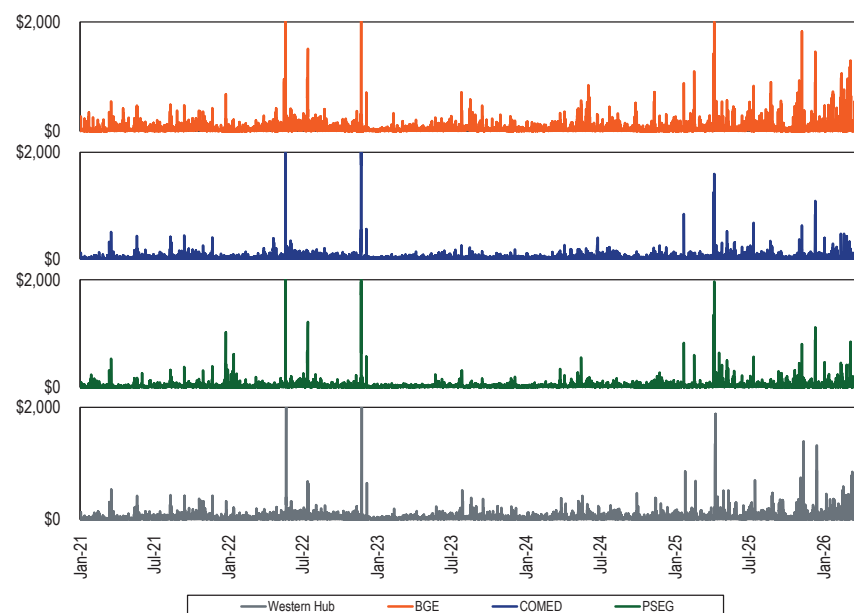
Figure 7-2 Hourly spark spread (gas) for peak hours ($/MWh): 2021 through June 2026 4
