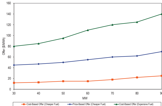
Figure 3-59 Dual fuel unit offers
