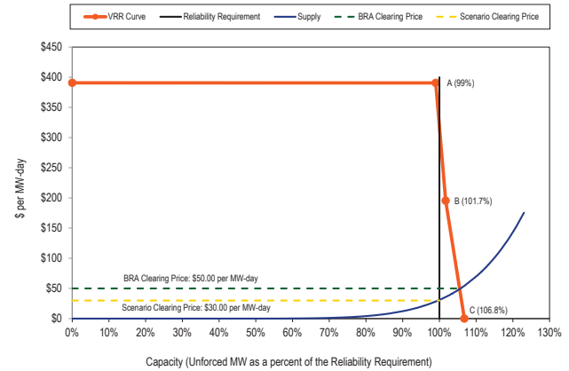
Figure 5-4 Shape of the VRR curve relative to the reliability requirement: 2022/2023 Delivery Year
