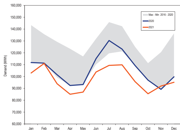
Figure 3-15 Day-ahead monthly average demand plus exports: 2020 through 2021
