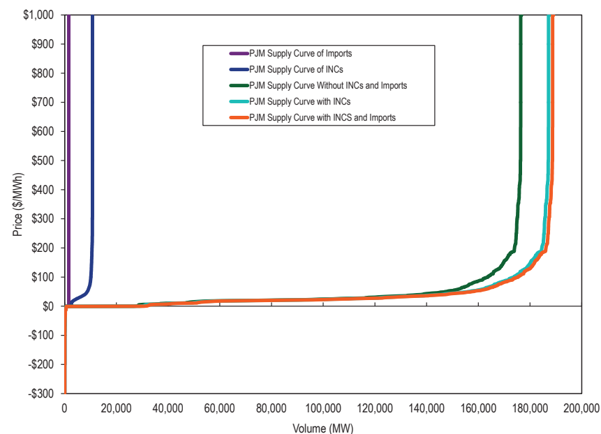
Figure 3-33 PJM day-ahead aggregate supply curves: 2017 example day
