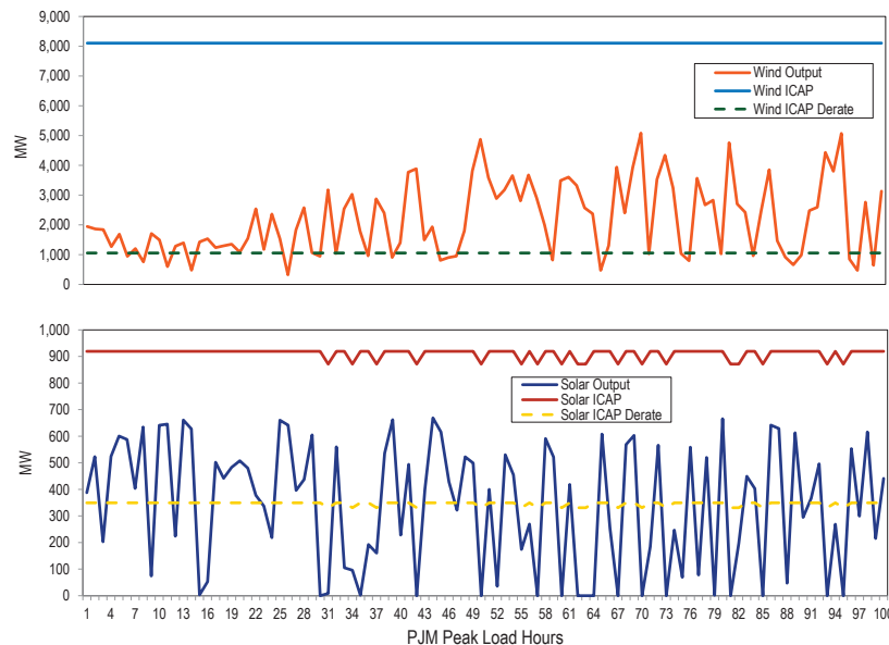
Figure 8-12 Wind and solar output during the top 100 peak load hours in PJM: January 1 through June 30, 2017
