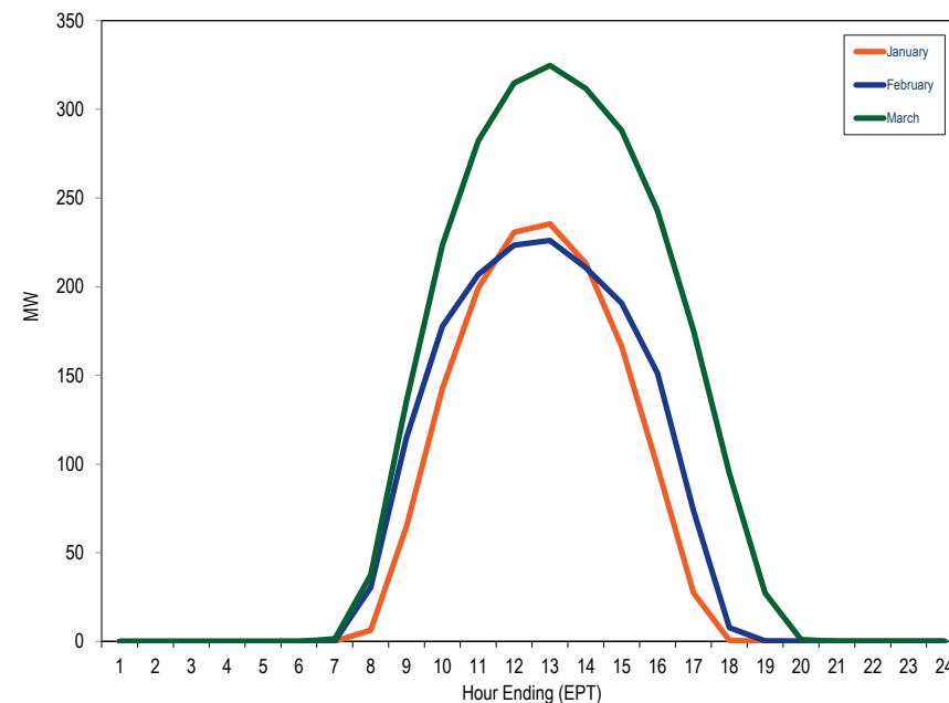
Figure 8-10 Average hourly real-time generation of solar units in PJM: January through March 2016
