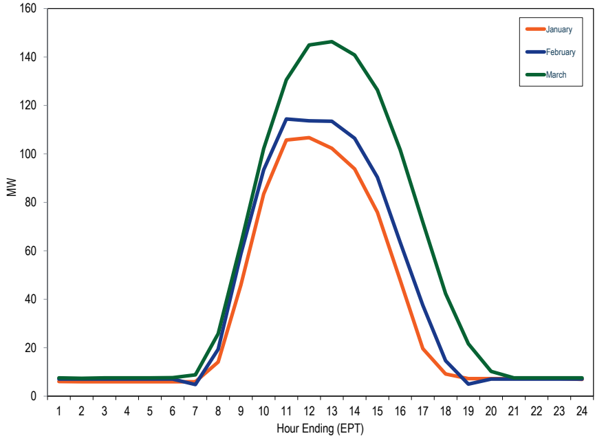
Figure 8-11 Average hourly day-ahead generation of solar units in PJM: January through March 2016
