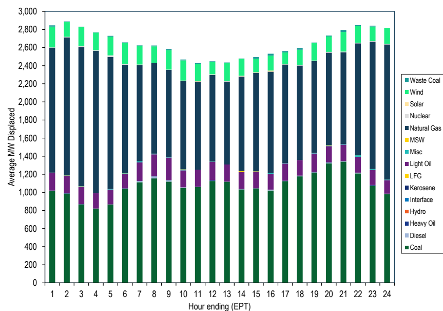
Figure 8-9 Marginal fuel at time of wind generation in PJM: January through March 2016
