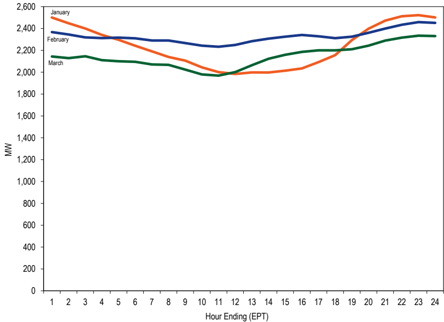
Figure 8-8 Average hourly day-ahead generation of wind units in PJM: January through March 2016
