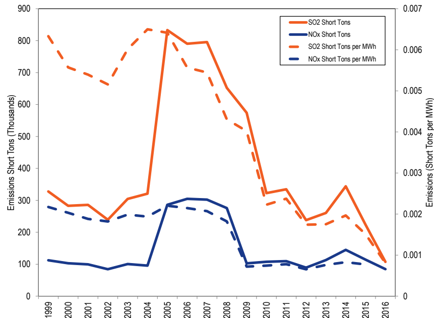
Figure 8-6 SO 2 and NO x emissions by year (thousands of short tons), by PJM units: January 1999 through March 2016 131
